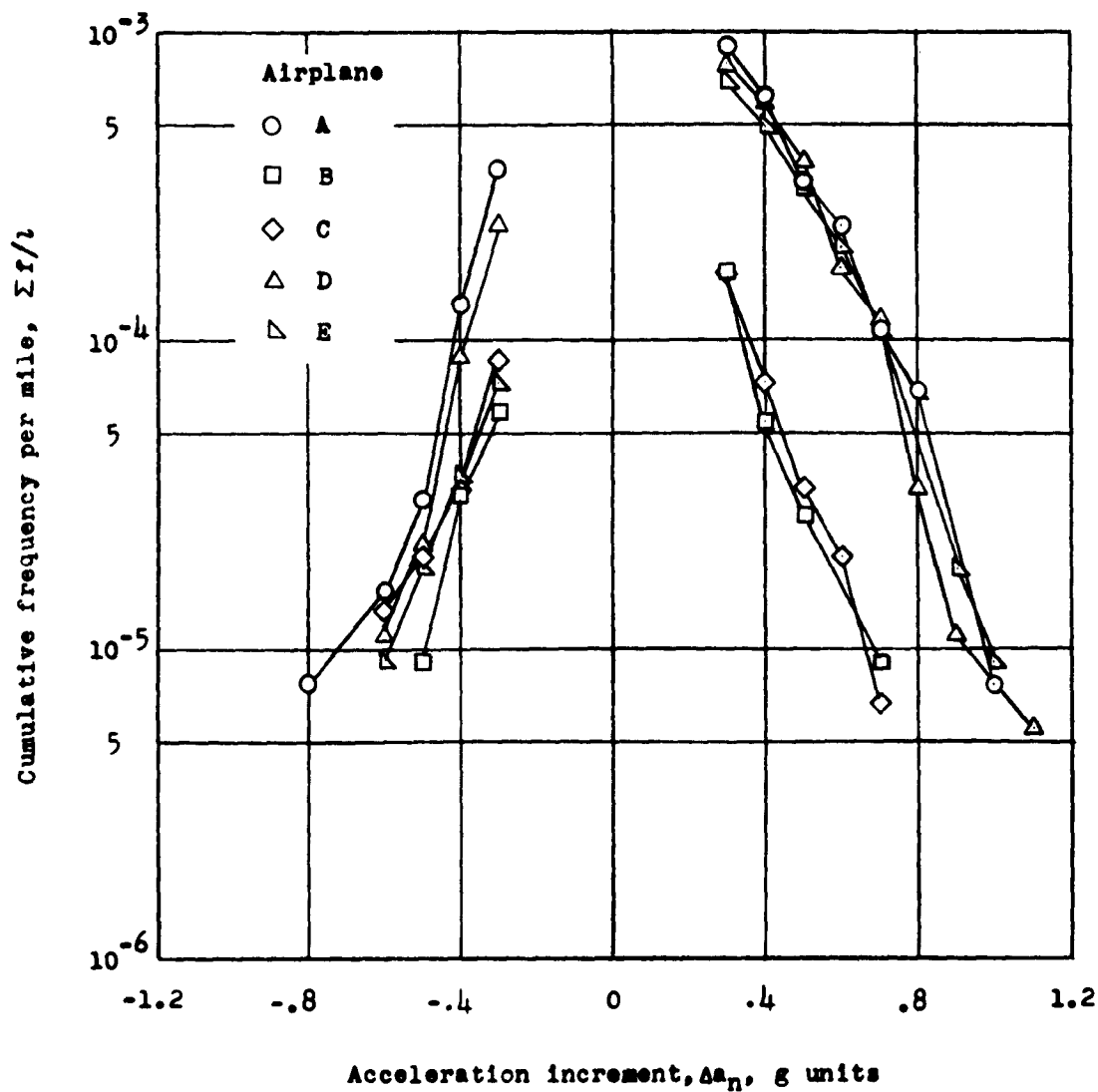
Figure 3.- Comparison of acceleration increments caused by check-flight maneuvers on five airplanes.
