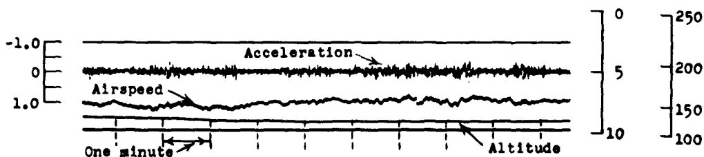
(b) Check-flight-maneuver accelerations.
