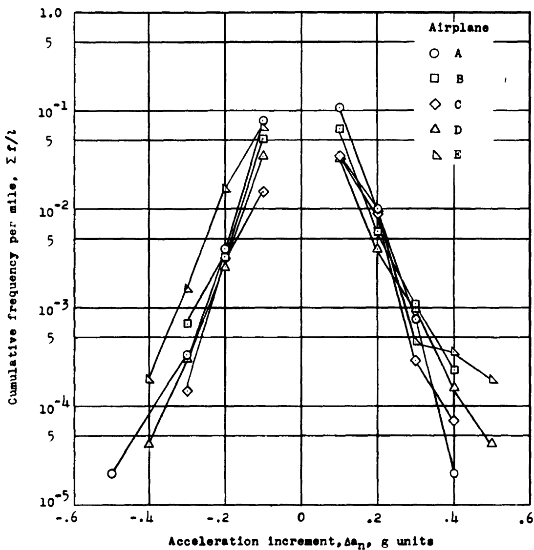
Figure 2.- Comparison of acceleration increments caused by operational maneuvers on five airplanes.
