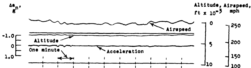
(a) Operational-maneuver accelerations.
