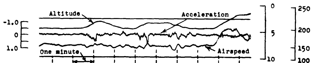
(b) Check-flight-maneuver accelerations.
