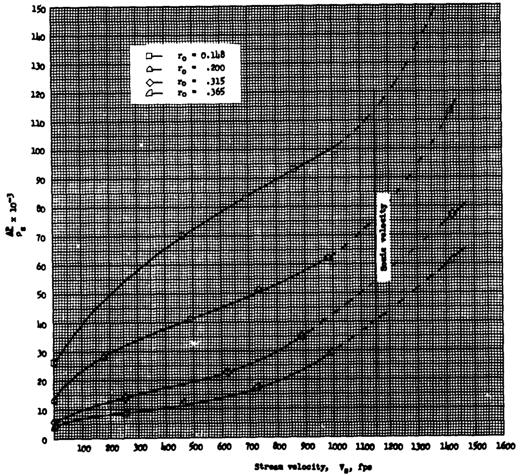
Figure 11.- Curves showing the manner in which \Delta P / \rho g varies with parallel-flow stream velocity for four perforated-material open ratios with a constant normal velocity of 30 fps. Symbols indicate cross-plot points.
