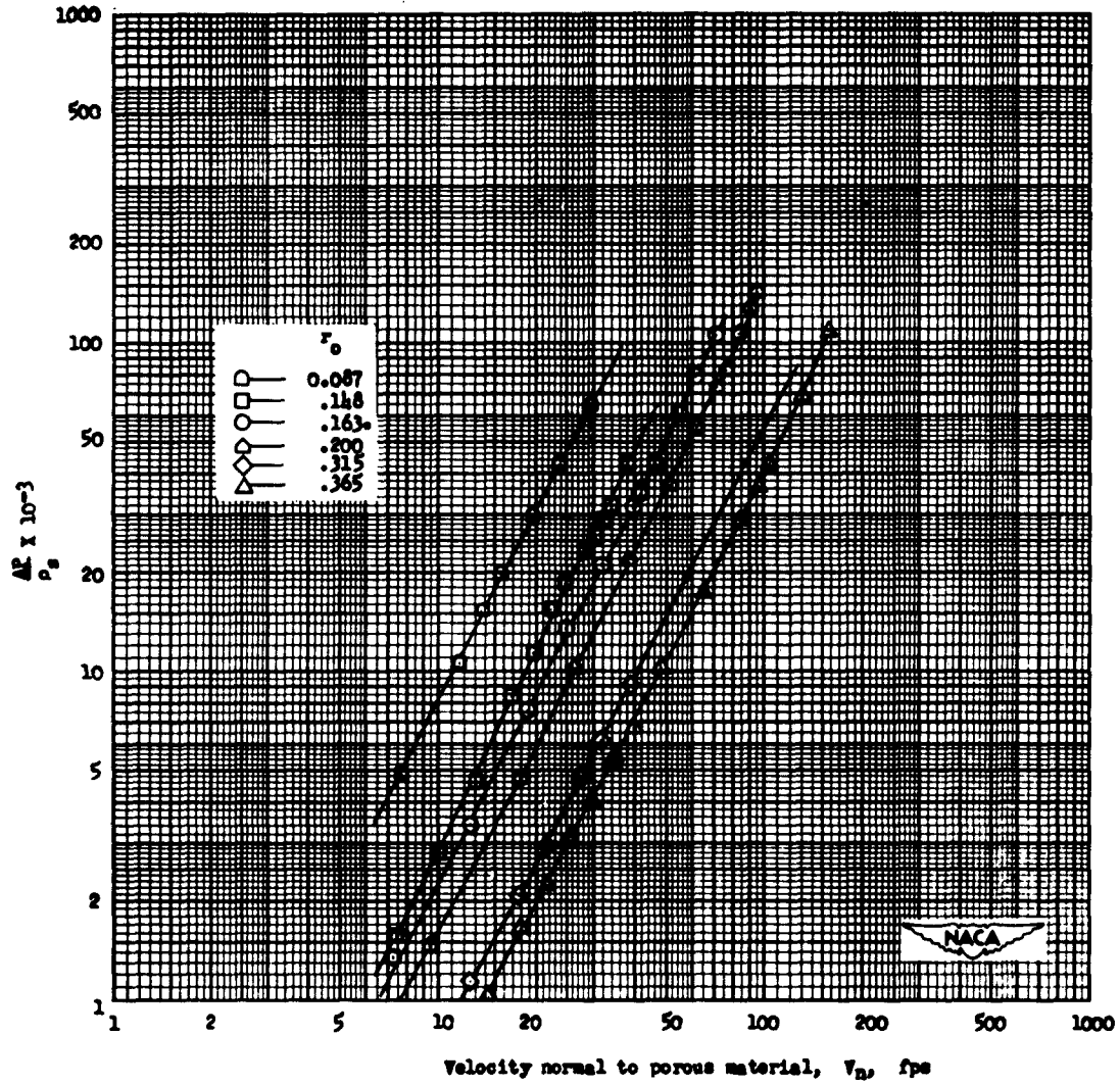
Figure 7.- Normal-flow calibration of perforated material for several different open ratios. \rho_s \approx 0.0022 slug/cu ft.
