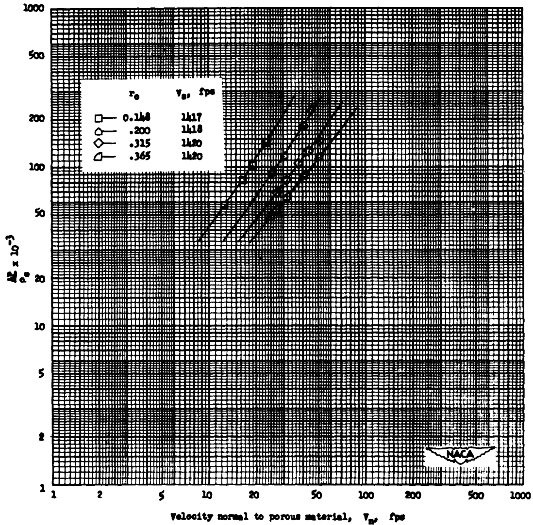
Figure 10.- Parallel-flow calibrations of four different open ratios in perforated material at a Mach number of approximately 1.3. \rho_s \approx 0.0009 slug/cu ft.
