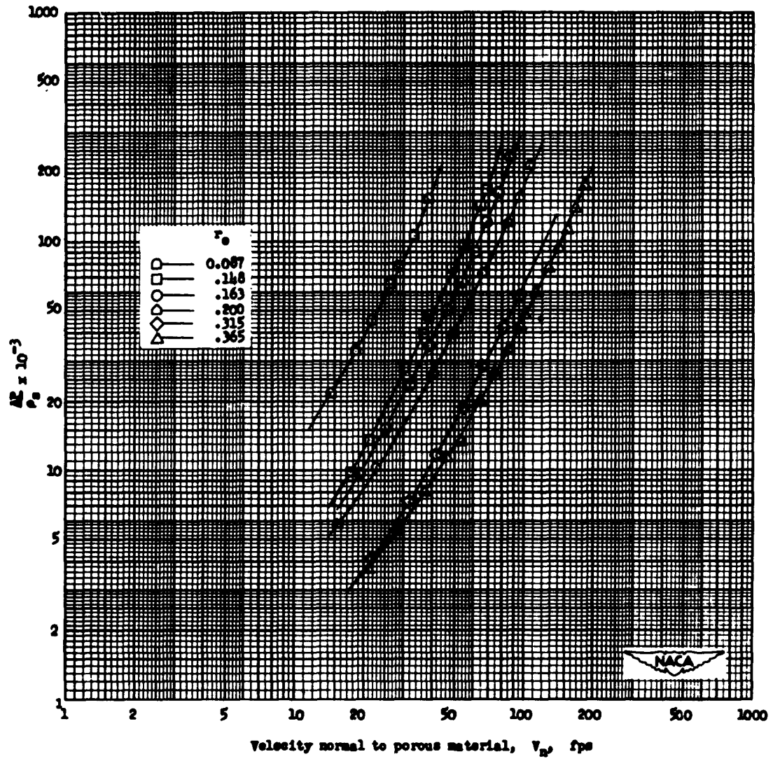
Figure 6.- Normal-flow calibration of perforated material for several different open ratios. \rho_s \approx 0.0009 slug / cu ft.
