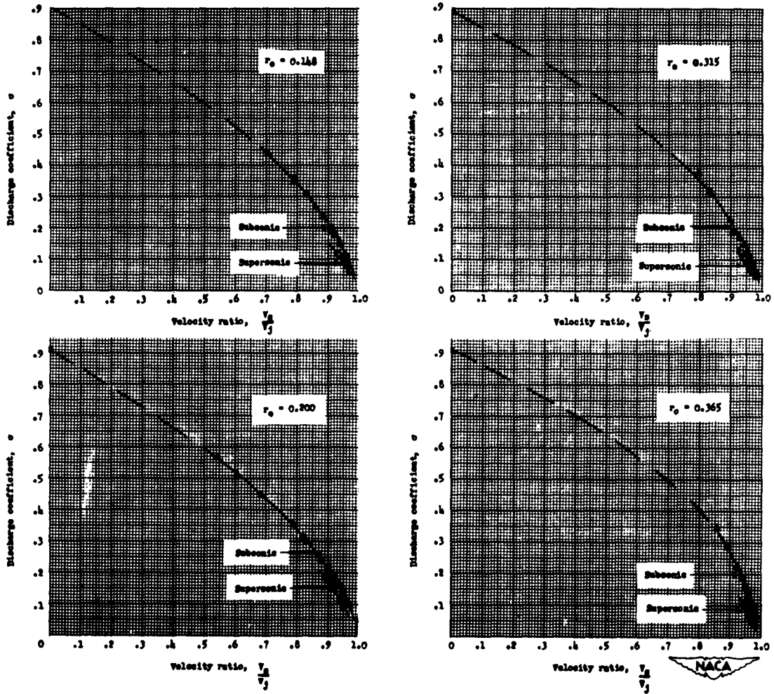
Figure 12.- Relation between discharge coefficient and velocity ratio for perforated material in parallel flow.
