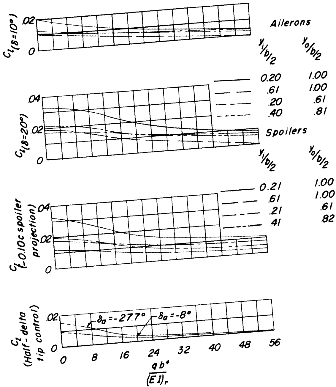
Figure 11.- Variation of rolling-moment coefficient with scaling factor for ailerons and spoilers on A_f -wing at \alpha = 0^\circ .
