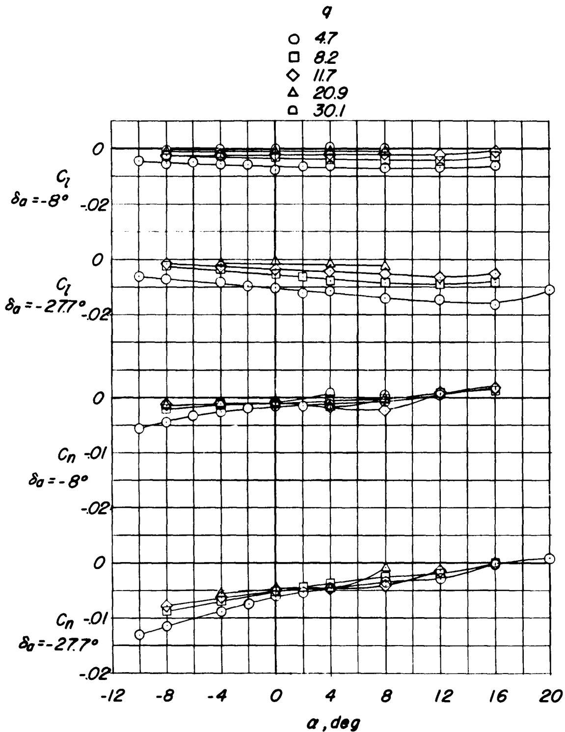
(e) Half-delta tip control.
