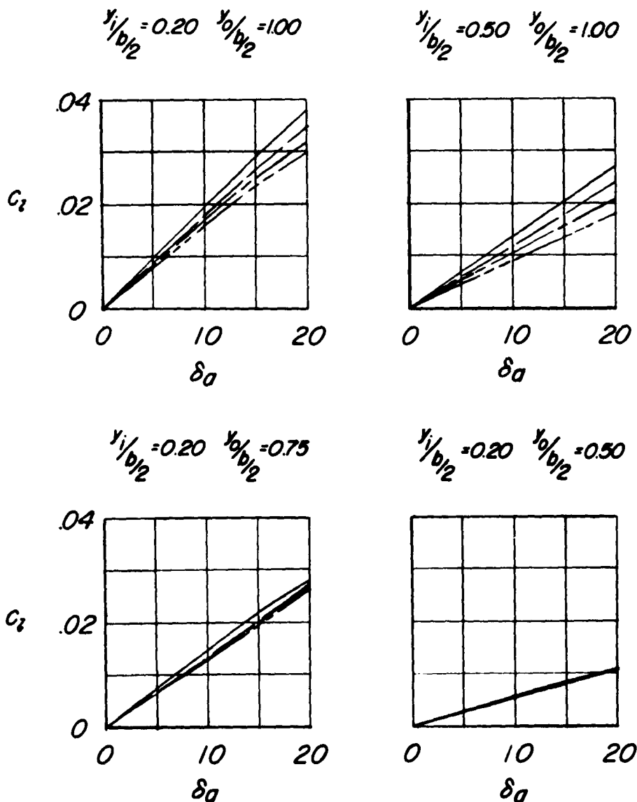
Figure 14.- Effects of dynamic pressure on variation of rolling-moment coefficient with aileron deflection for various spans of ailerons on the M_F -wing at \alpha = 0^\circ .
