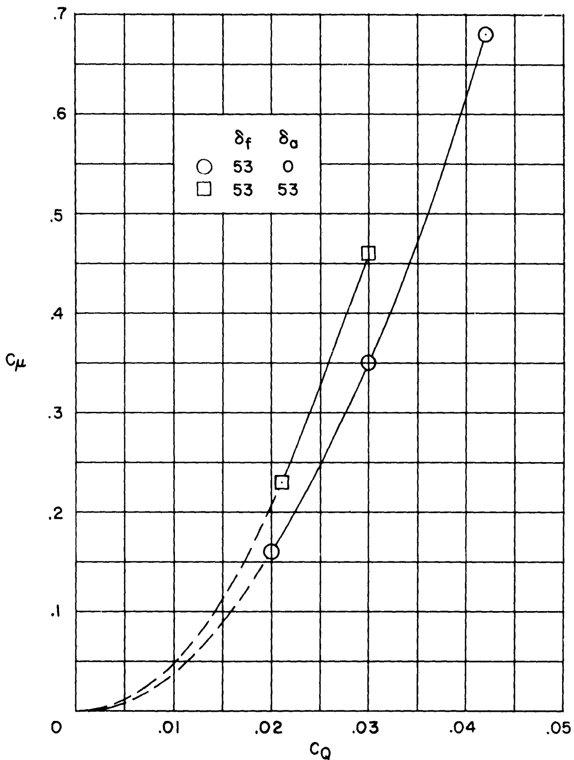
Figure 22.- Variation of the momentum coefficient with the quantity of flow coefficient.
