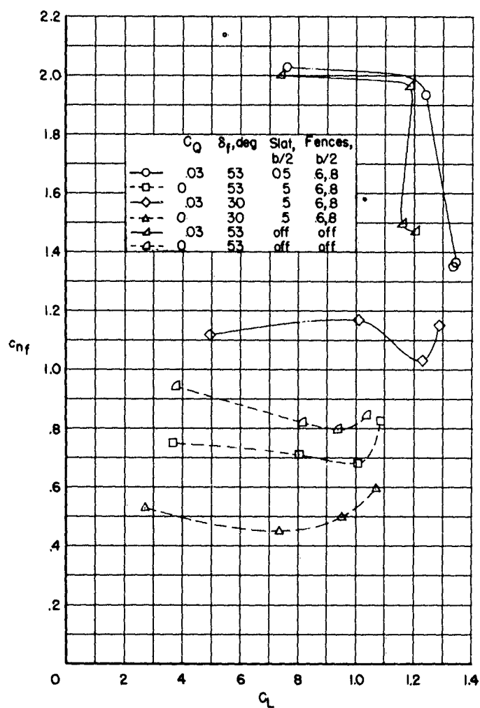
(b) c_{nf} against C_L .
