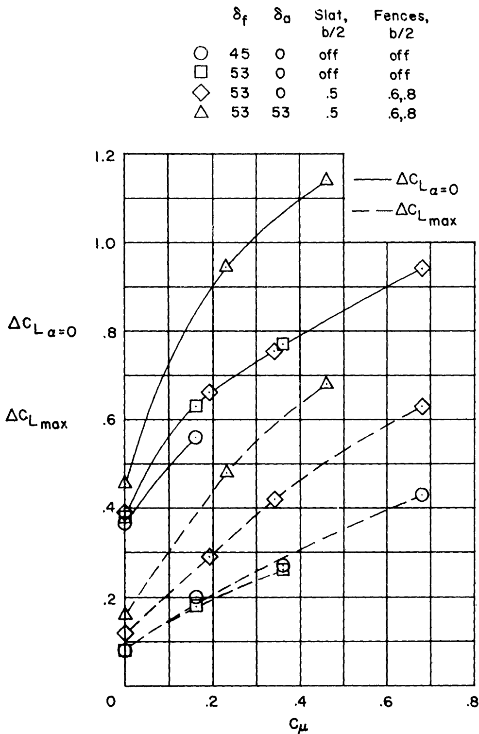
Figure 21.- Summary of the effect on \Delta C_{L_{\alpha=0}} and \Delta C_{L_{max}} of momentum coefficient, flap deflection, aileron deflection, and a slat and fences.
