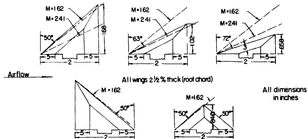
(a) Wing models illustrating Mach cone leading-edge configuration.
