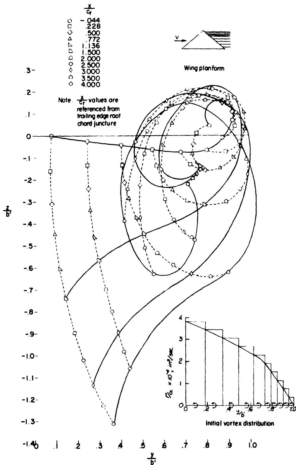
Figure 49.- Theoretical paths of ten infinite line vortices behind the straight 0-taper-ratio wing ( \Lambda = -\Lambda_{TE} = 50^\circ ). M = 1.62 ; R = 1.42 \times 10^6 ; \alpha = 9^\circ .
