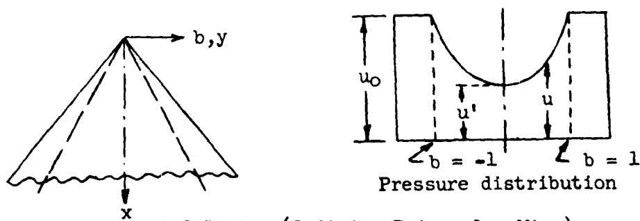
SKETCH I. (Infinite Triangular Wing)
