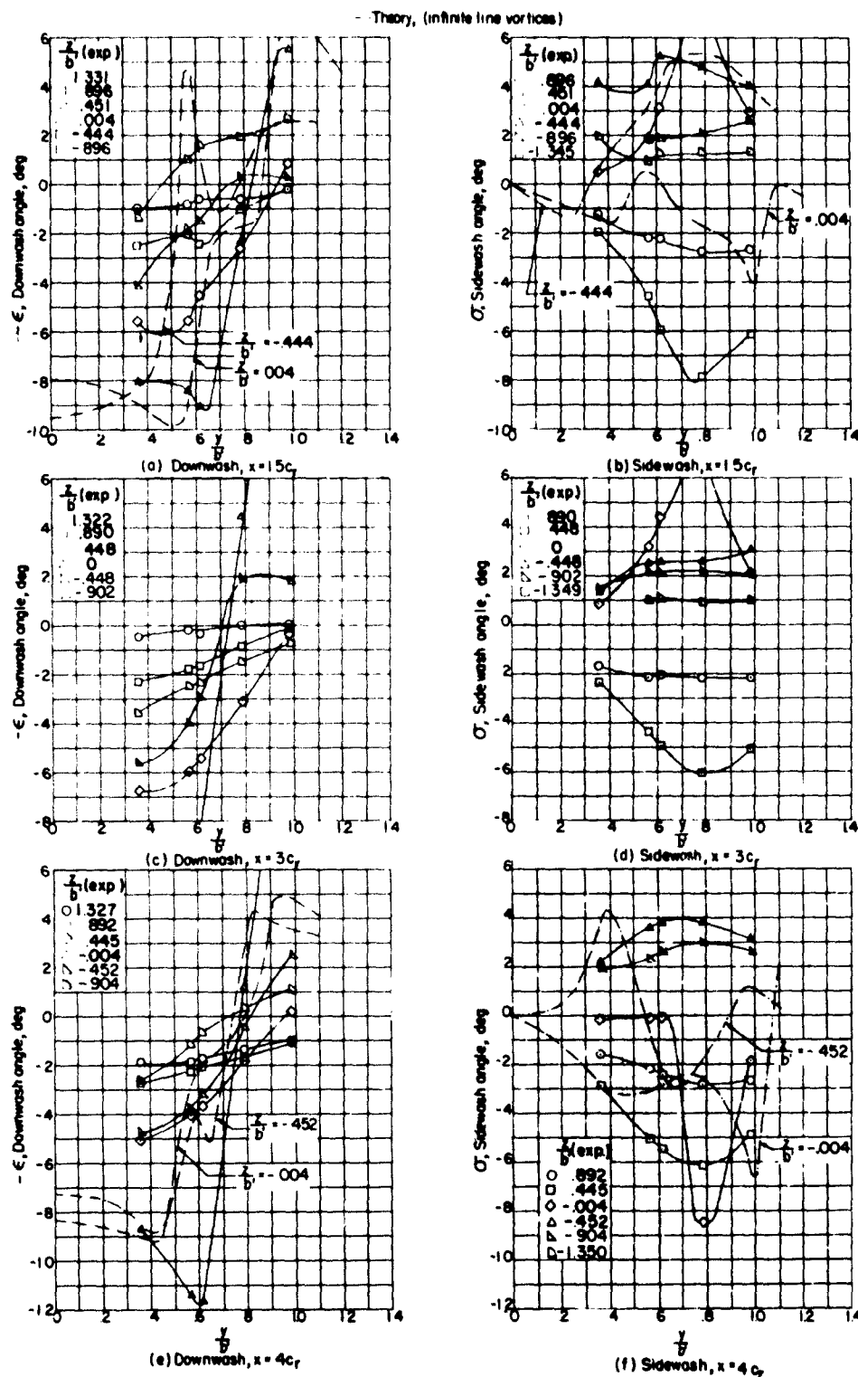
Figure 50.- Spanwise variation of the downwash and sidewash behind the straight O-taper-ratio wing ( \Lambda = -\Lambda_{TE} = 50^\circ ). M = 1.62 ; R = 1.42 \times 10^6 ; \alpha = 9^\circ .
