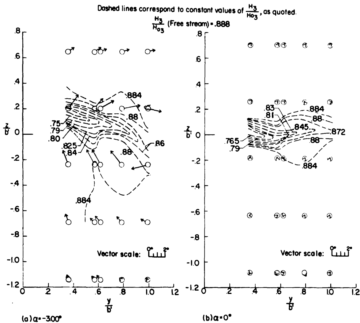
Figure 30.- Pressure contours and vector representation of the flow behind a straight O-taper-ratio wing. \Lambda = -\Lambda_{TE} = 50^\circ ; M = 1.62 ; x = 1.5c_r ; R = 1.42 \times 10^6 .
