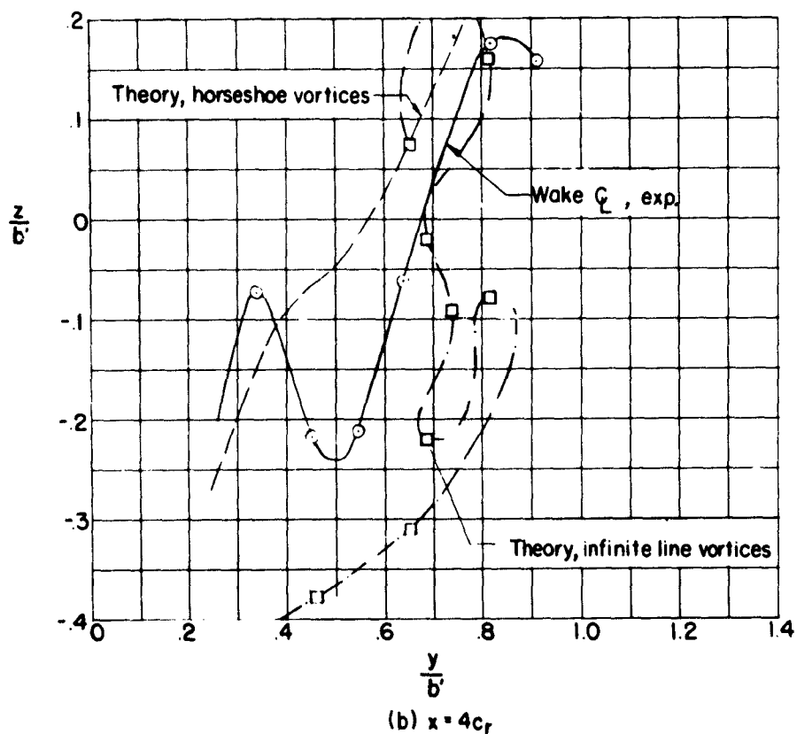
Figure 44.- Wake center-line location and comparison with various theories for the 50° sweptback triangular wing. M = 2.41 .
