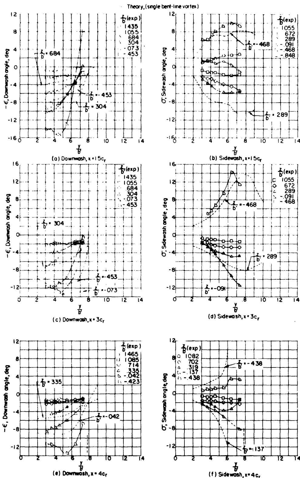
Figure 41.- Spanwise variation of downwash and sidewash for 72^\circ sweptback triangular wing. M = 2.41 ; R = 1.42 \times 10^6 ; \alpha = 17^\circ .
