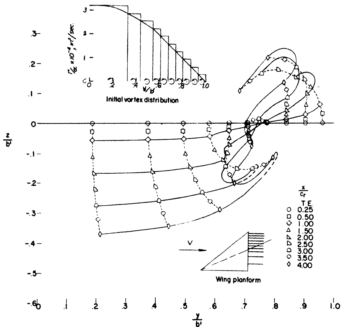
Figure 45.- Theoretical paths of ten infinite line vortices behind the 50° sweptback triangular wing. M = 2.41 ; \alpha = 12^\circ .
