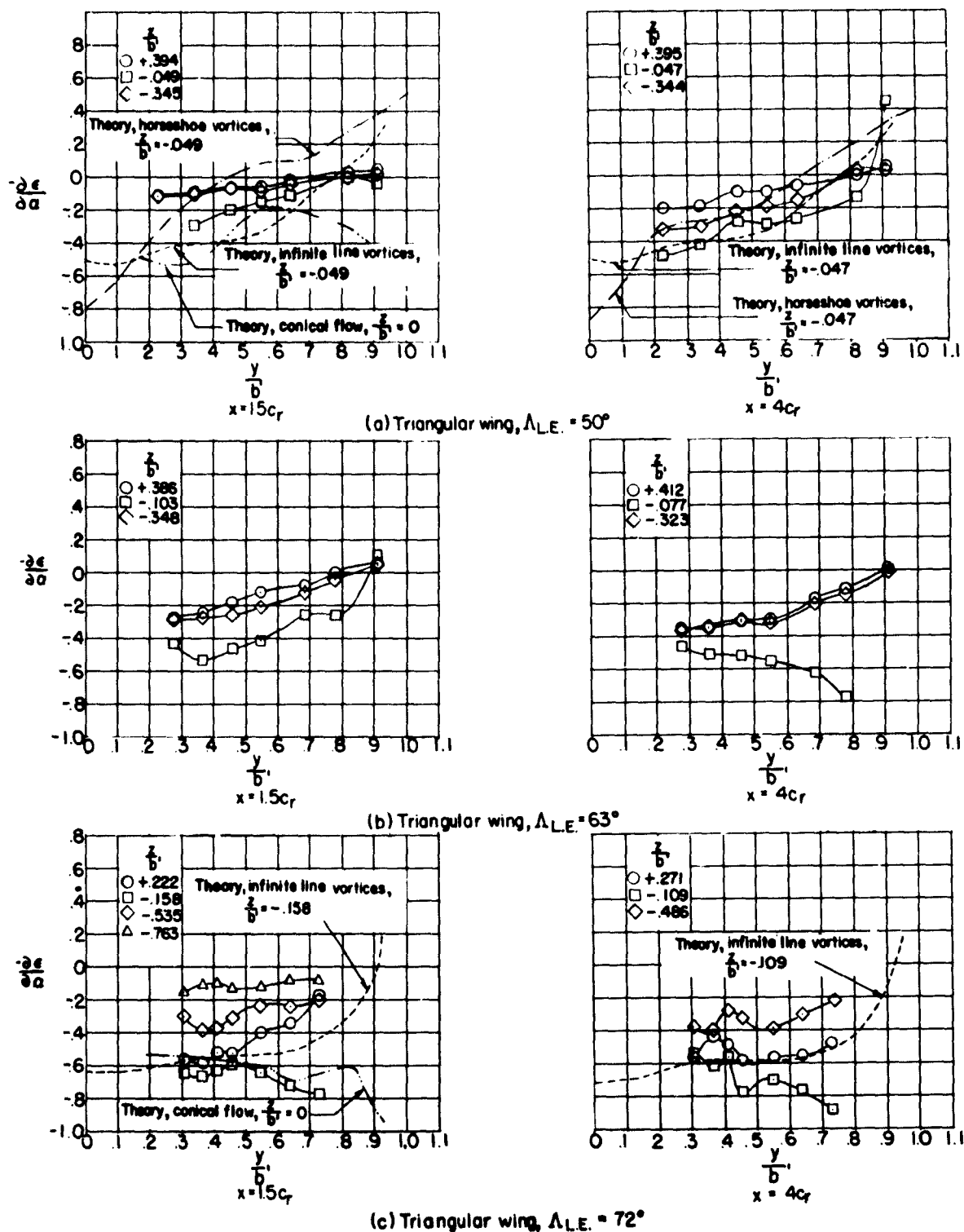
Figure 33.- Spanwise variation in -\frac{\partial \epsilon}{\partial \alpha} near \alpha = 0^\circ (\pm 3^\circ) for three triangular wings. M = 2.41 ; R = 1.42 \times 10^6 .
