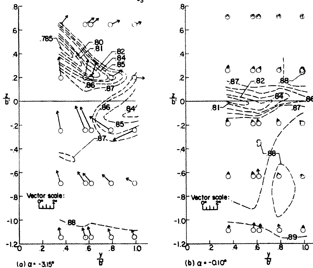
Figure 32.- Pressure contours and vector representation of the flow behind a straight 0-taper-ratio wing. \Lambda = -\Lambda_{TE} = 50^\circ ; M = 1.62 ; x = 4c_r ; R = 1.42 \times 10^6 .
