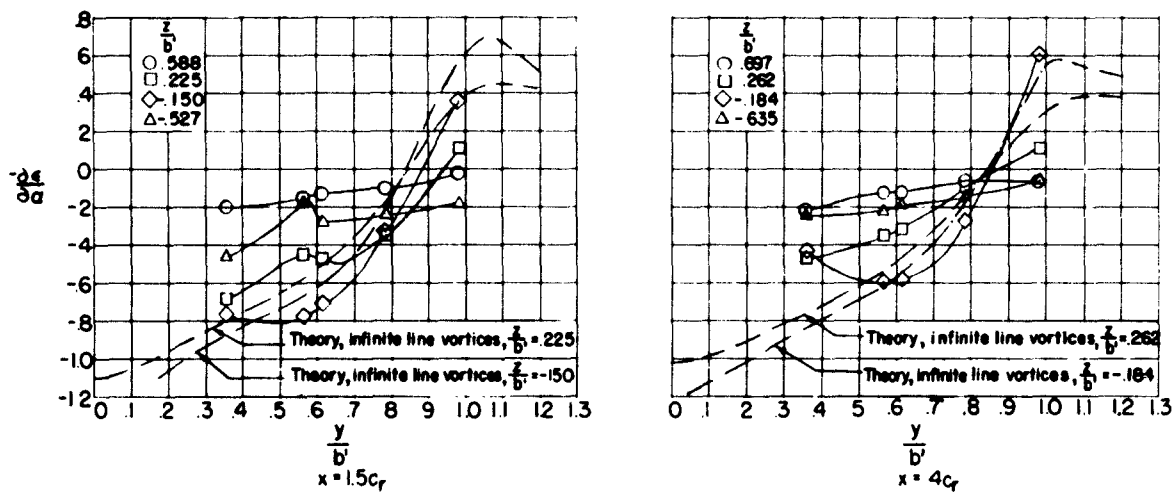
(b) 0 Taper wing, \Delta L_E = \Delta T_E = -50^\circ
