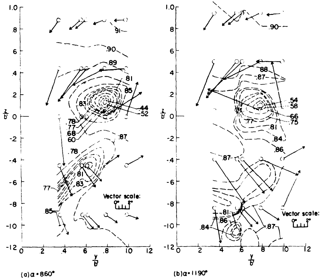
Figure 31.- Pressure contours and vector representation of the flow behind a straight 0-taper-ratio wing. \Lambda = -\Lambda_{TE} = 50^\circ ; M = 1.62 ; x = 3c_r ; R = 1.42 \times 10^6 .
