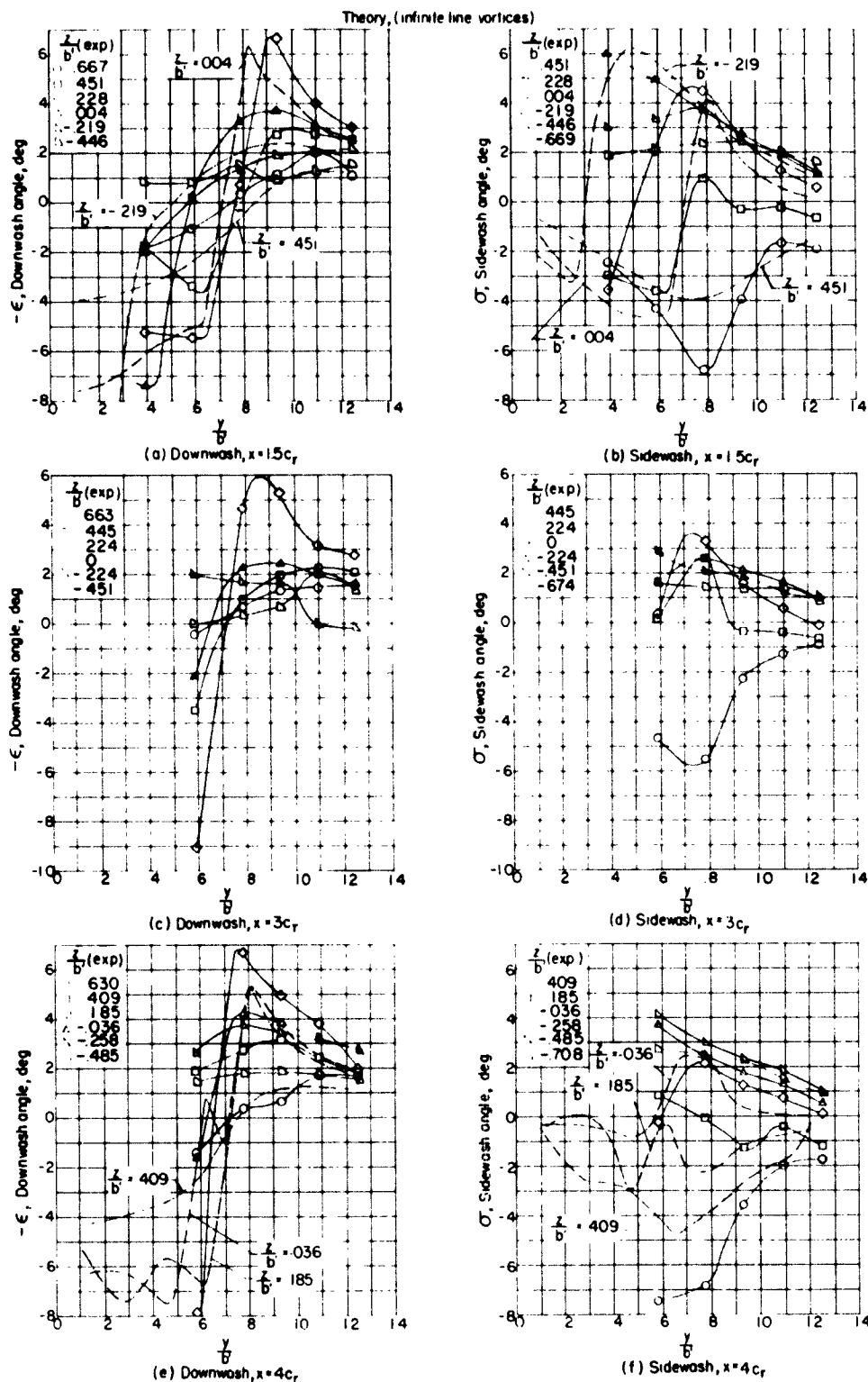
Figure 48.- Spanwise variation of the downwash and sidewash for the reversed triangular wing ( \Lambda_{TE} = -50^\circ ). M = 1.62 ; R = 1.42 \times 10^6 ; \alpha = 9^\circ .
