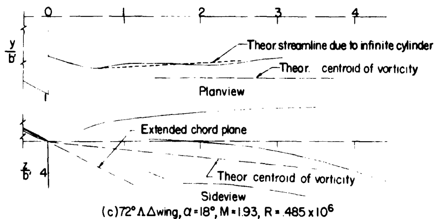
Figure 4.- Sketches illustrating the locations of the paths of high vorticity behind triangular wings.
