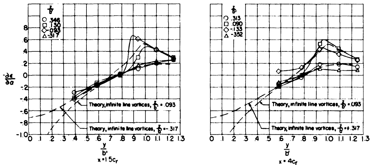
(a) Reversed triangular wing, \Delta T_E = -50^\circ
