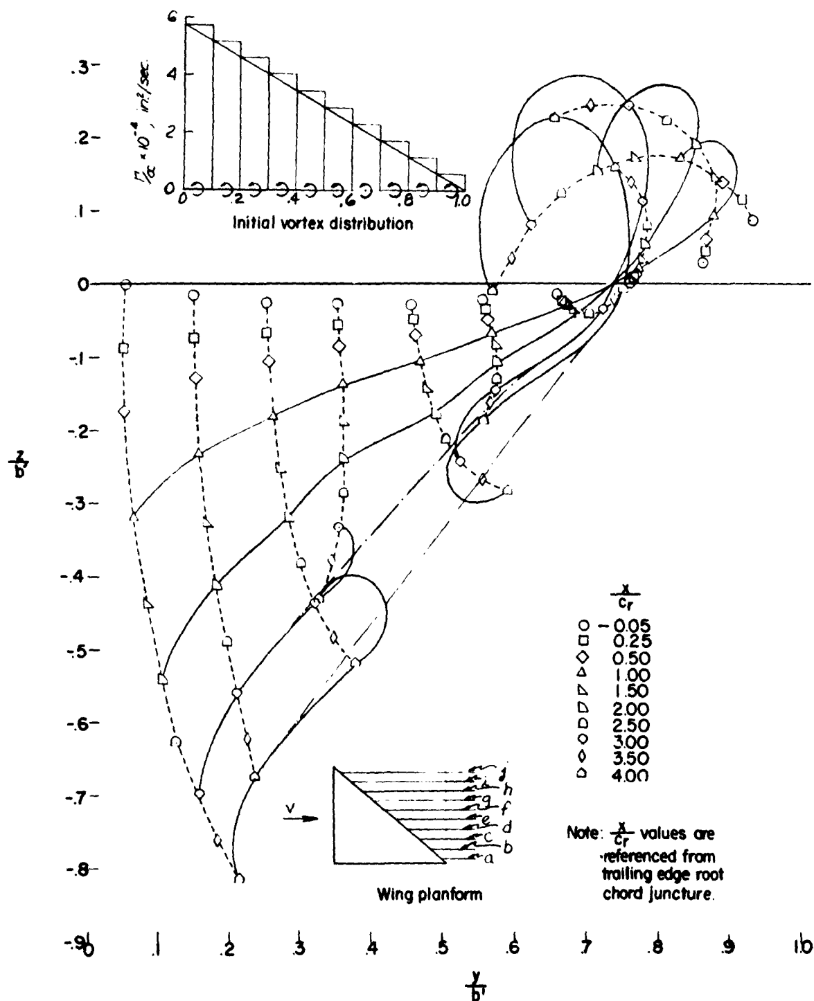
Figure 47.- Theoretical paths of ten infinite line vortices behind the reversed triangular wing. M = 1.62 ; \alpha = 9^\circ .
