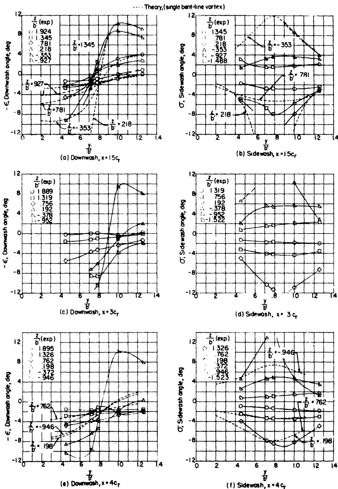
Figure 42.- Spanwise variation of downwash and sidewash for 72^\circ sweptback triangular wing. M = 1.62 ; R = 1.42 \times 10^6 ; \alpha = 17^\circ .
