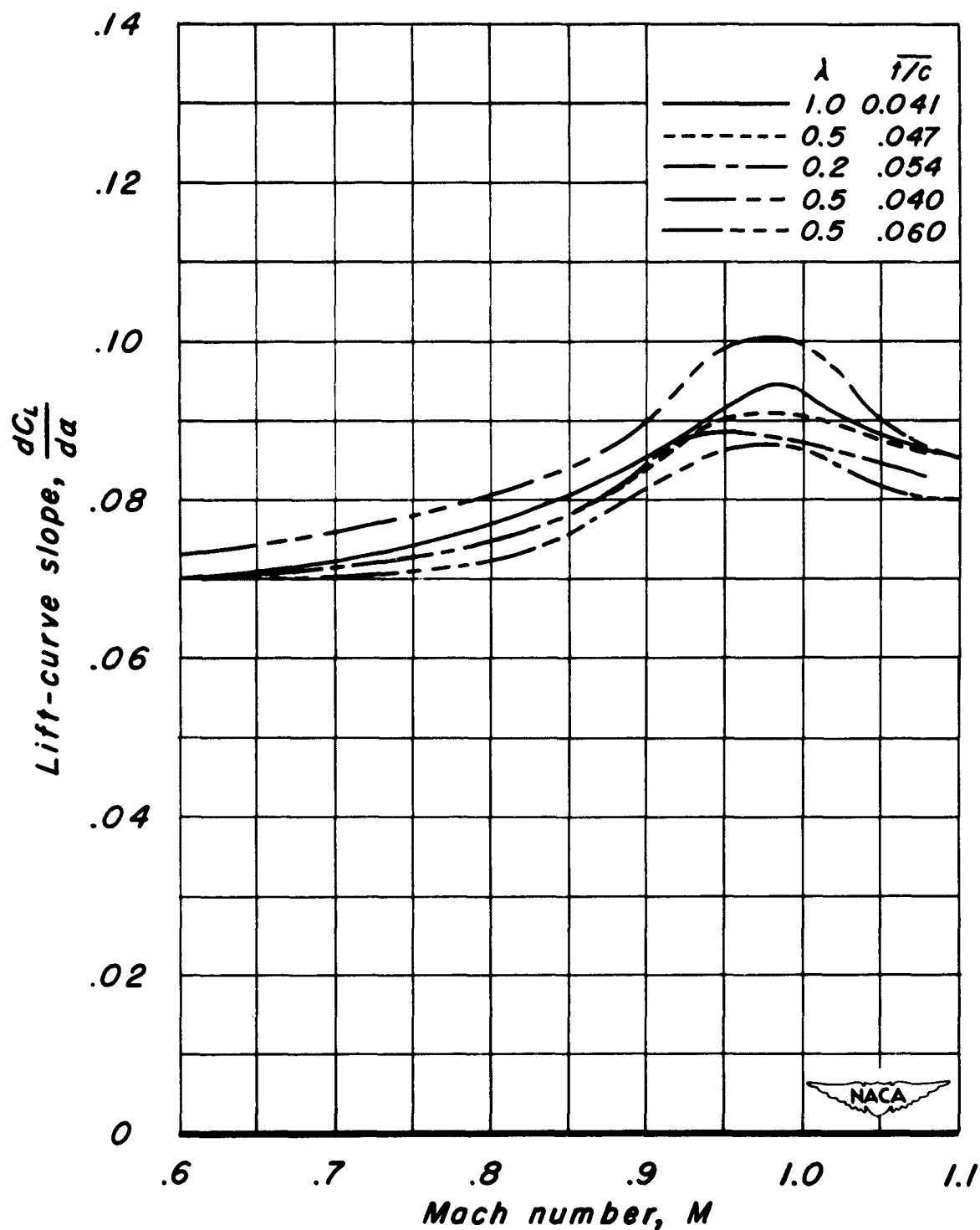
Figure 10.- The variation of lift-curve slope with Mach number.
