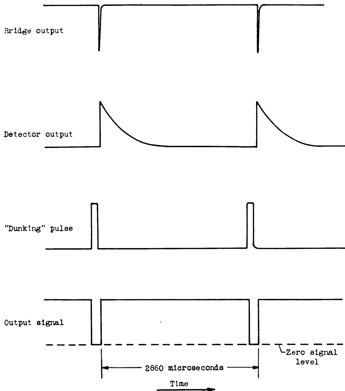
Figure 5. - Wave forms.
