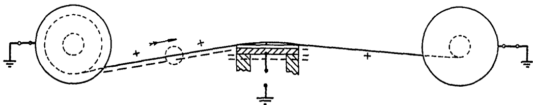
(b) DISTRIBUTION OF SURPLUS CHARGE WITH INSULATED FRICTION SURFACE.
