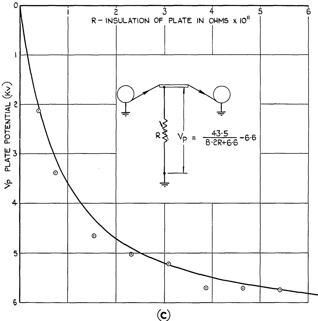
FIG.8(a, b&c) VARIATION OF POTENTIAL OR CHARGE DENSITY ON PLATE RUBBING SURFACE WITH CHANGE OF PLATE INSULATION TO EARTH.
