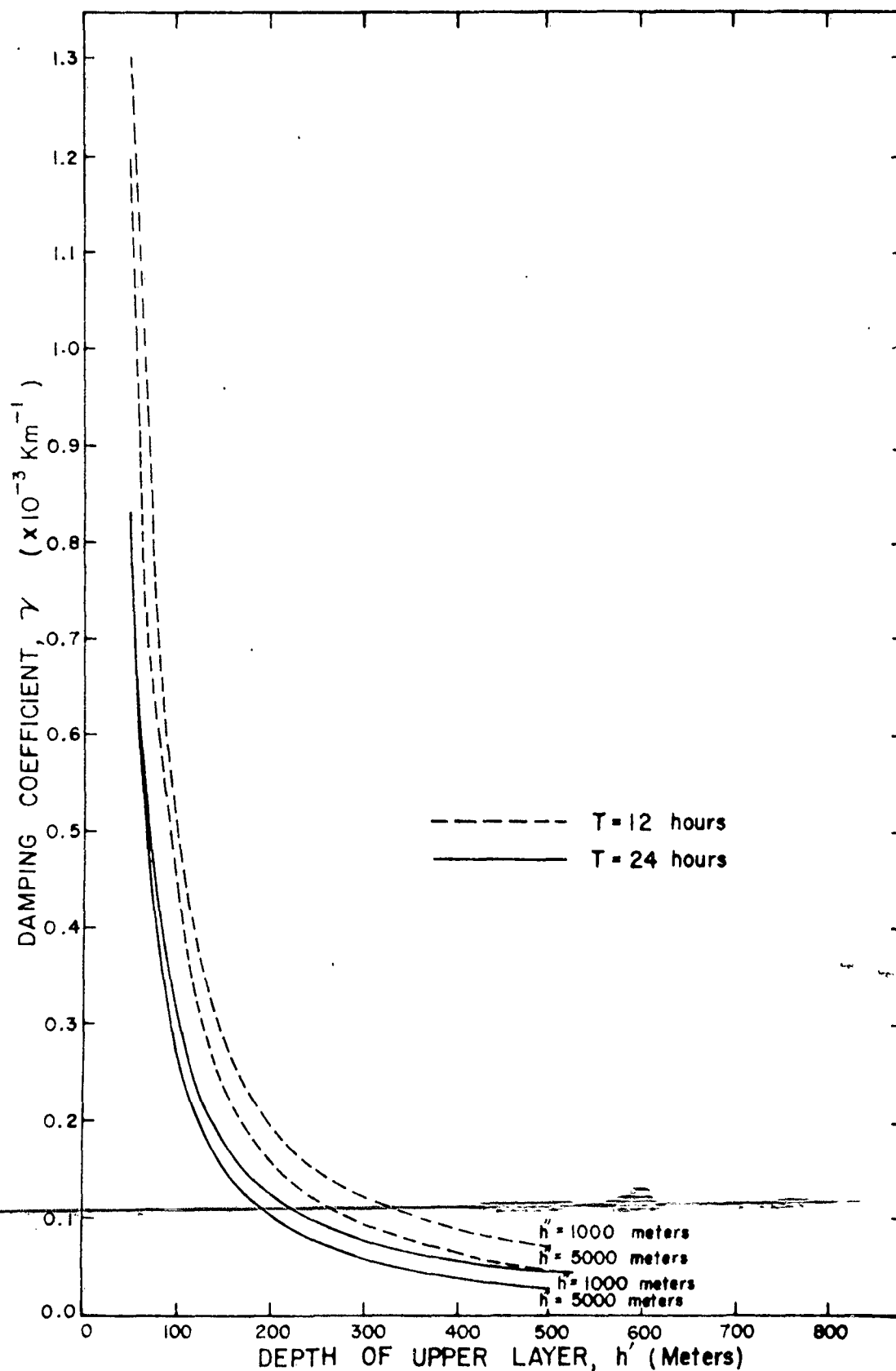
FIGURE 1. Damping Coefficient Variation with Layer Depth (L = 15^\circ, \gamma = 1 \text{ cm}^2 \text{ sec}^{-1}, \Delta \rho = 10^{-3} \text{ gms. cm}^{-3}) .
