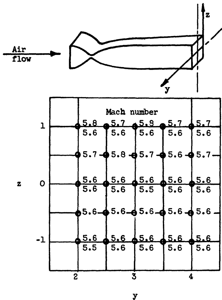
Figure 5. - Mach number calibration 33\frac{3}{4} inches downstream of throat of Lewis 6- by 6-inch hypersonic tunnel.
