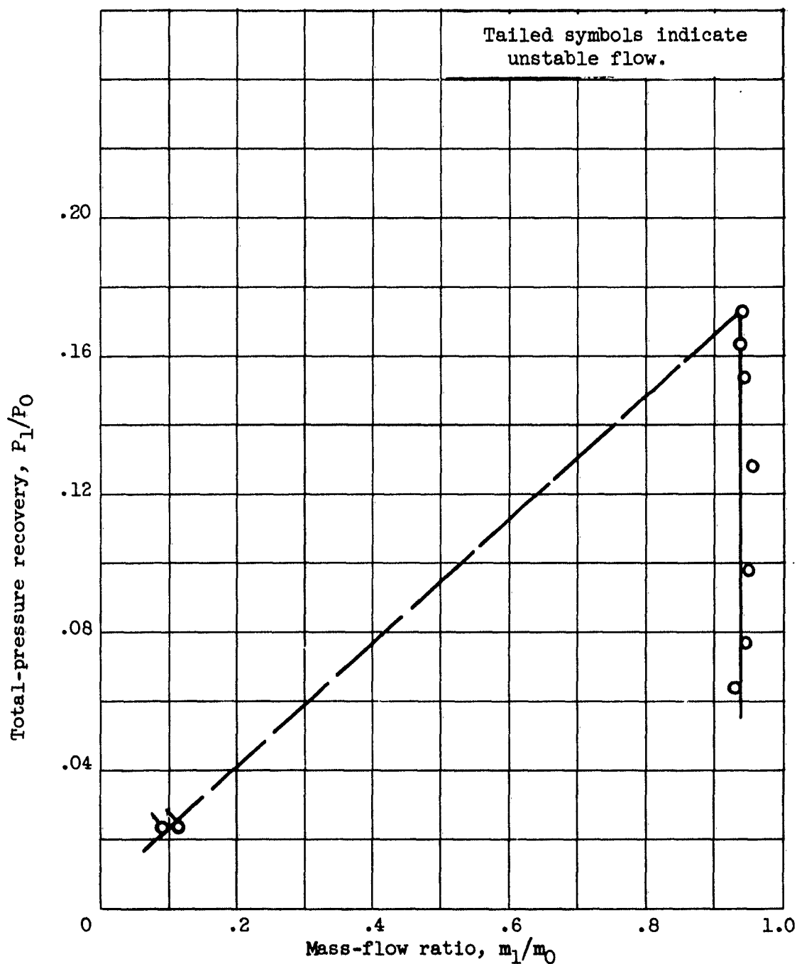
Figure 8. - Diffuser performance at 3^\circ angle of attack. Cowl A; forebody A; zero forebody translation; no roughness.
