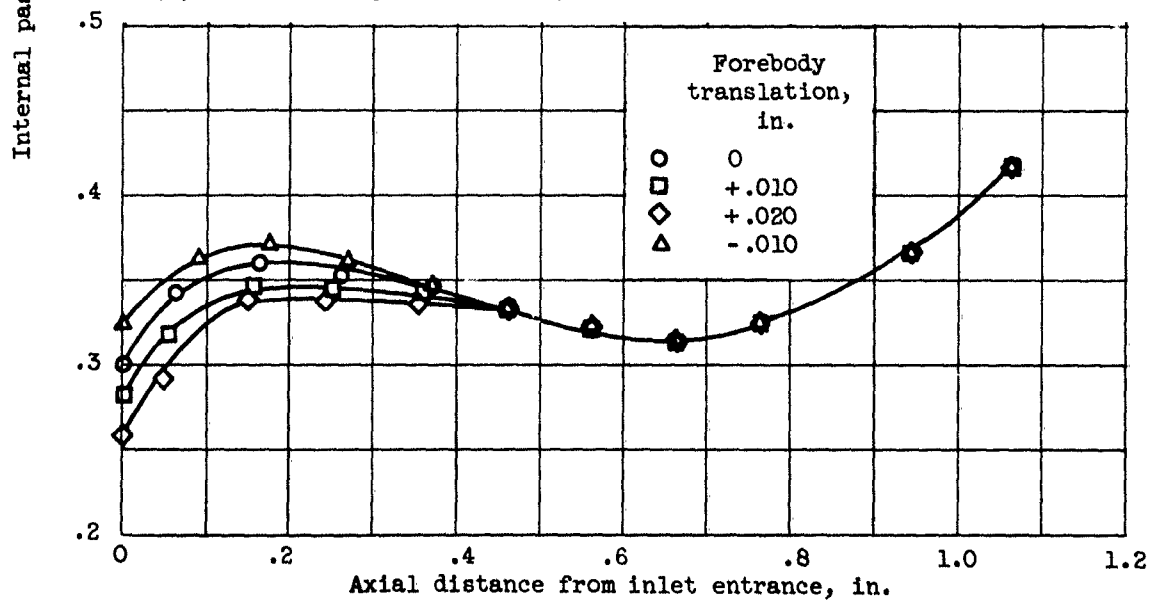
(b) Cowl B; forebody A; effects of forebody translation.
