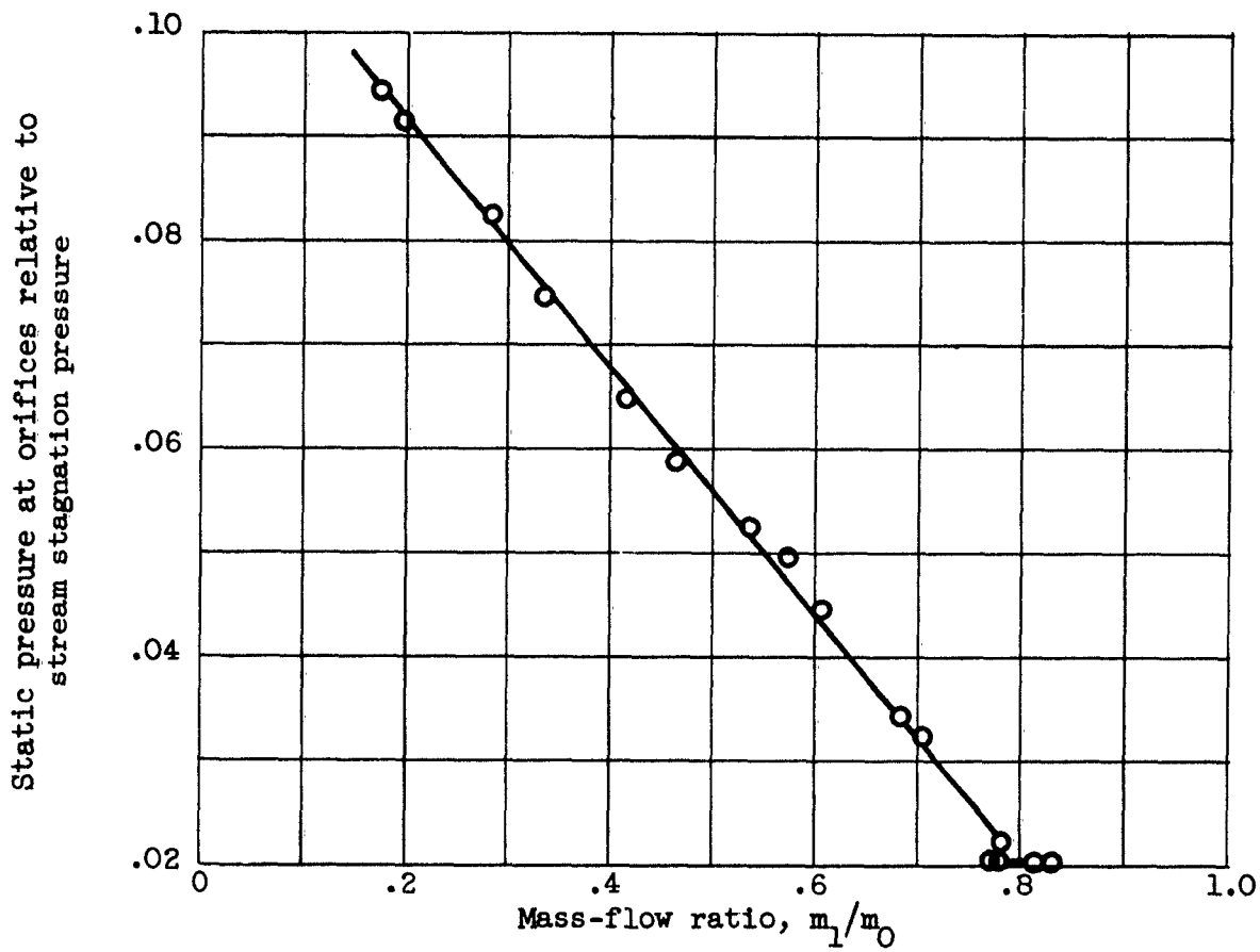
Figure 20. - Typical variation of measured static pressure at forebody orifices.
