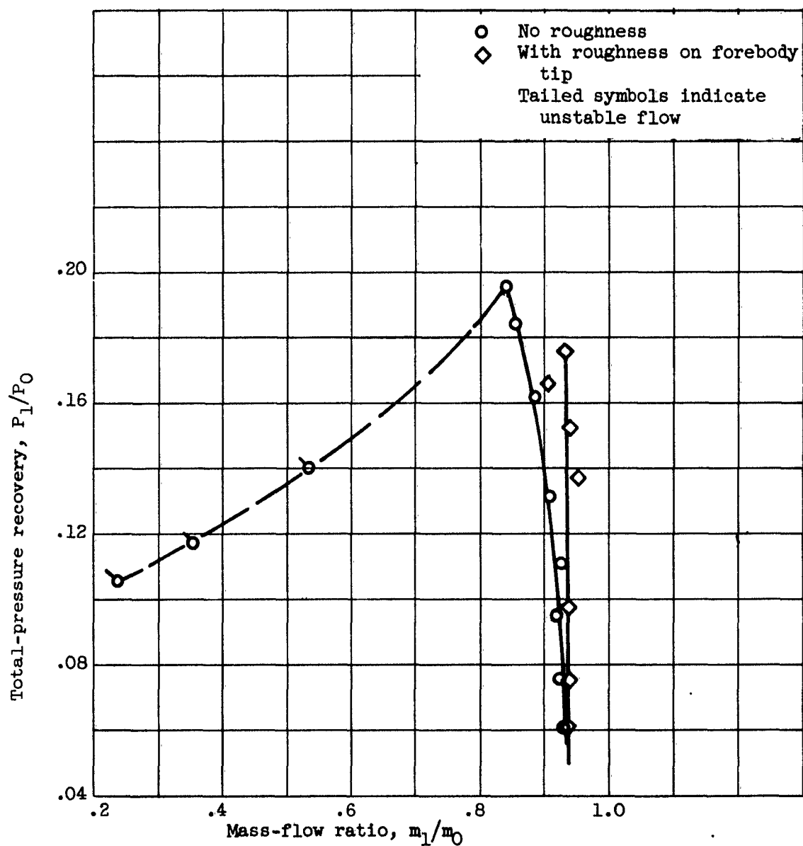
Figure 7. - Diffuser performance at zero angle of attack. Cowl A; forebody A; zero forebody translation.
