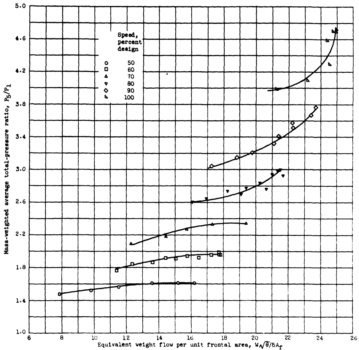
(a) Mass-weighted average total-pressure ratio.
