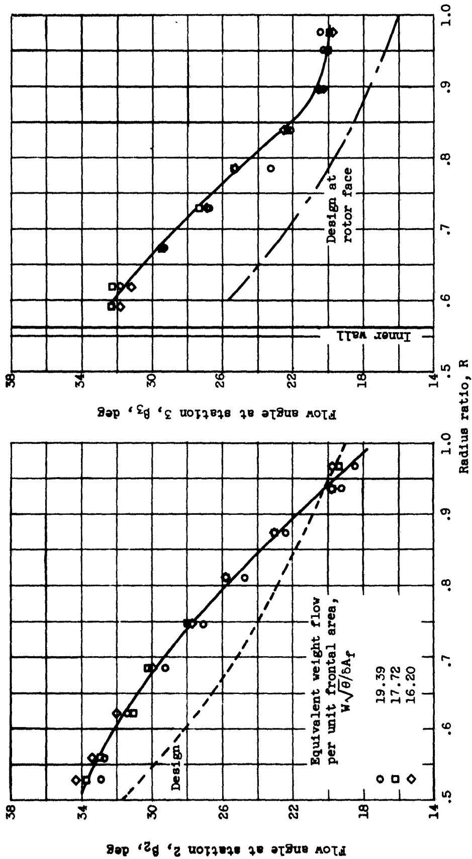
Figure 10. - Angle distribution behind guide vanes and in front of rotor.
