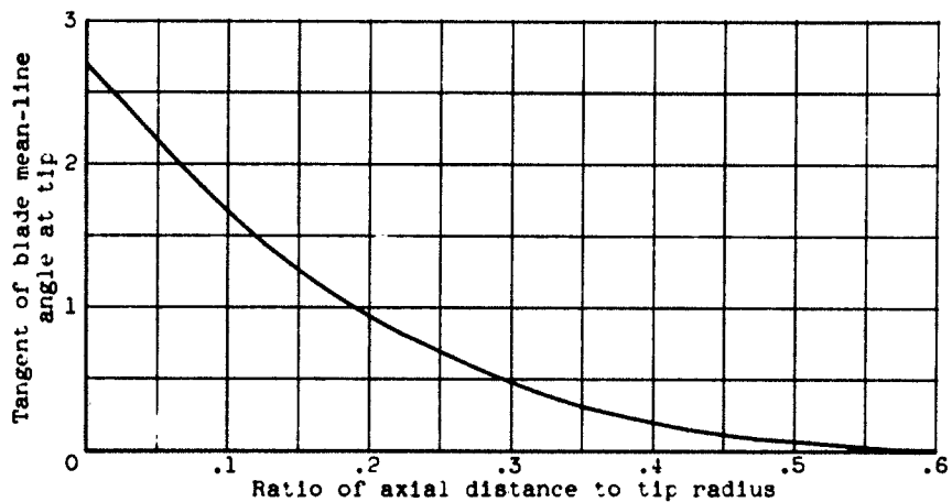
Figure 2. - Prescribed mean flow direction at tip.
