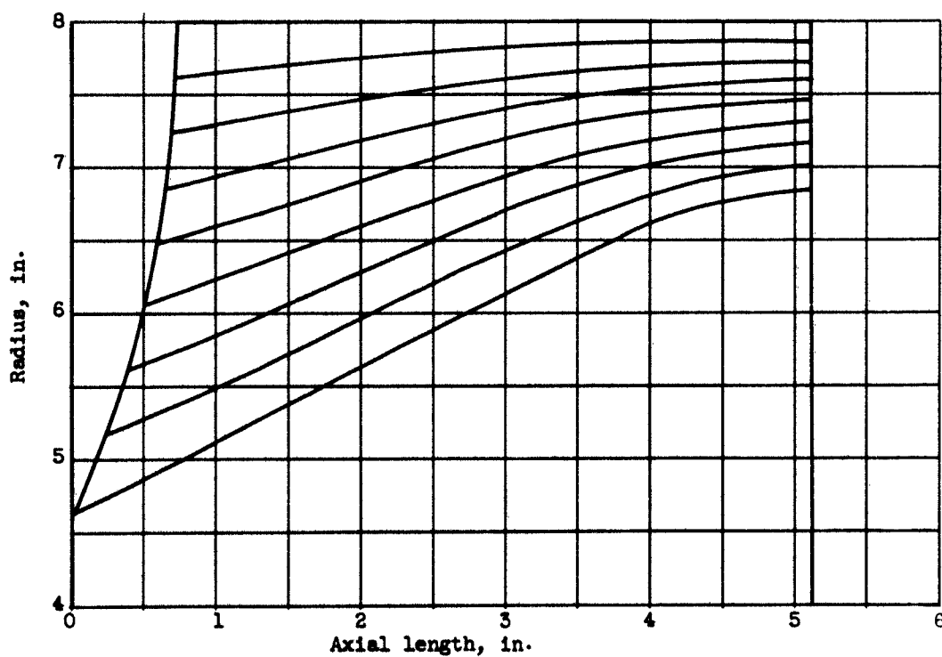
Figure 4. - Meridional section and blade layout of rotor.
