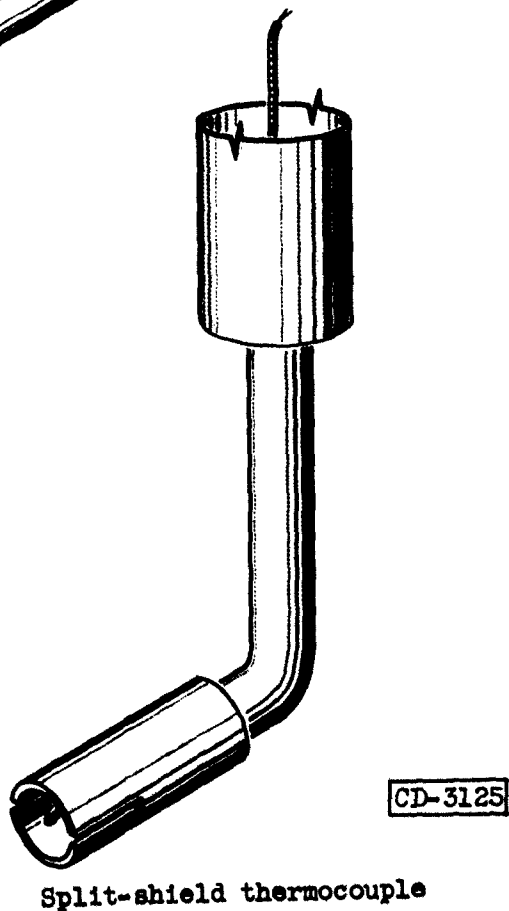
Figure 8. - Schematic sketches of instruments used in tests of rotor.
