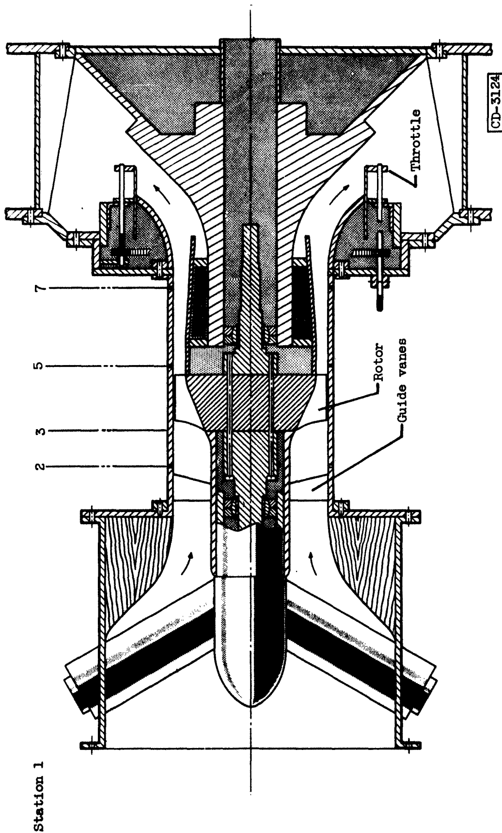
Figure 7. - Schematic sketch of rotor installed in variable-component test rig.
