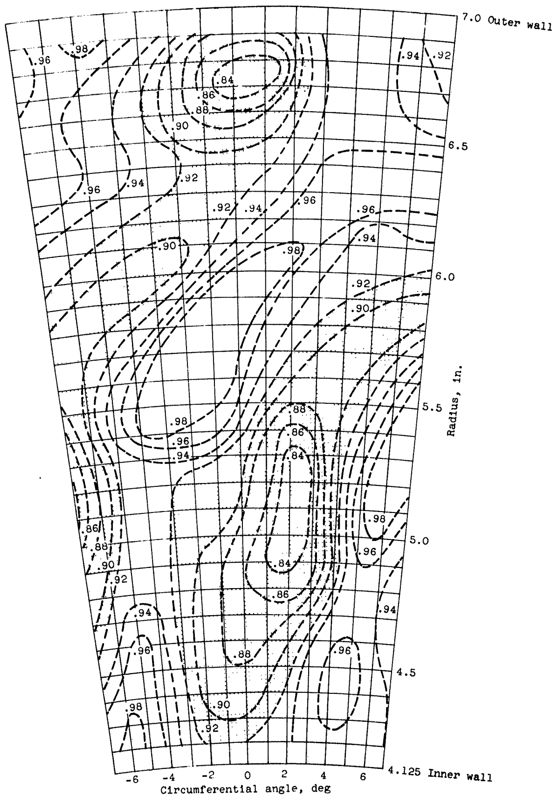
Figure 5. - Contours of local adiabatic efficiency \eta_B at station 3.
