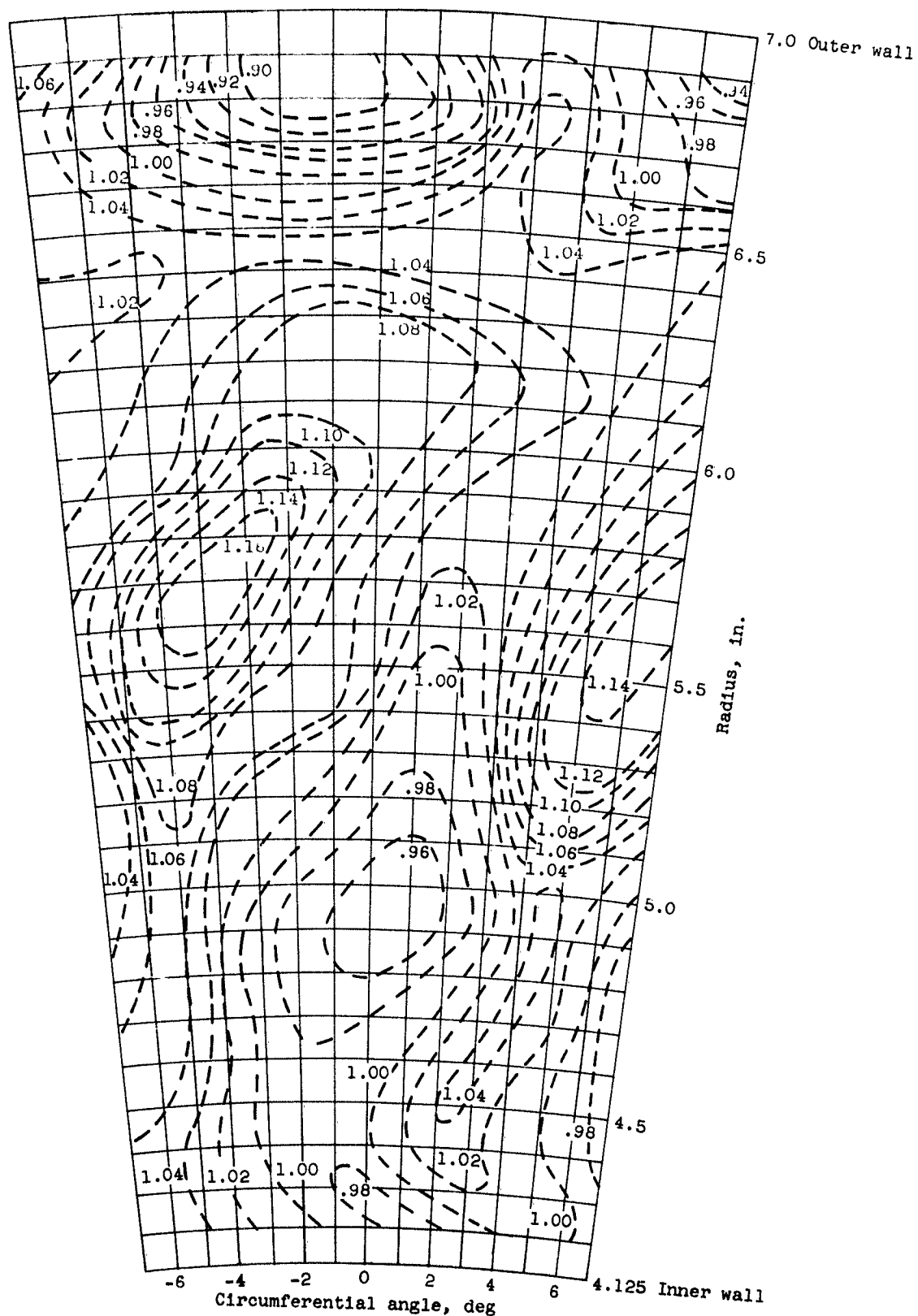
Figure 4. - Contours of corrected total-temperature-drop ratio (\Delta T/\theta)/(\Delta T/\theta)_{des} over survey range.
