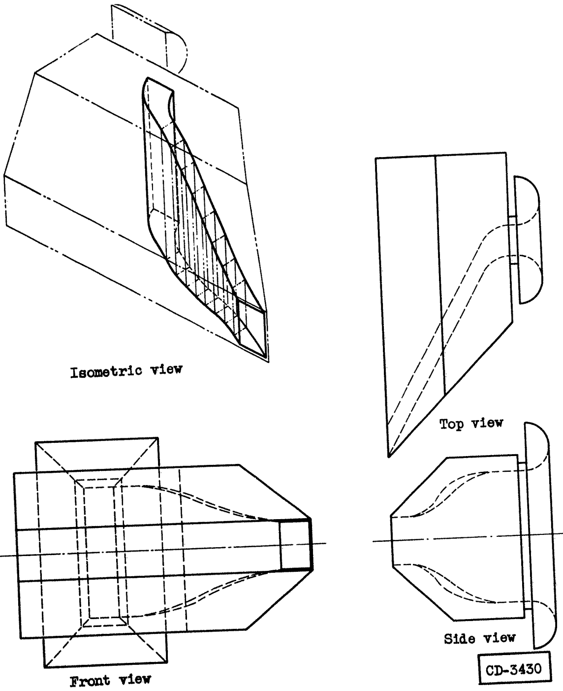
(c) Nozzle 3 (low-velocity-turning nozzle).
