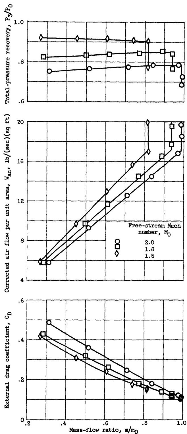
Figure 4. - Continued. Performance of 20-series inlets at zero angle of attack.
