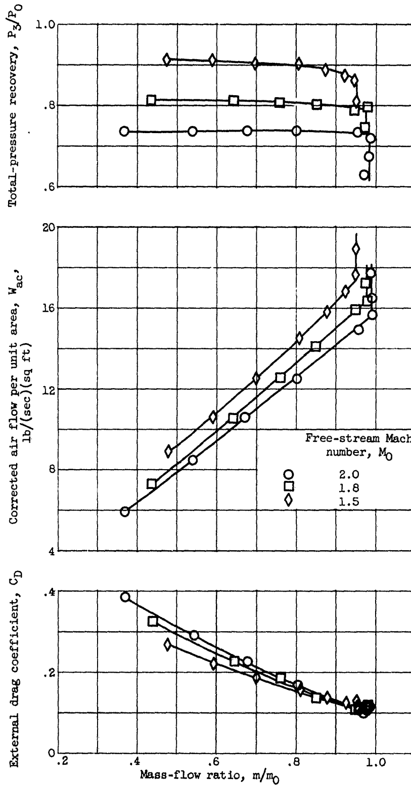
Figure 6. - Concluded. Performance of 15-series inlets at zero angle of attack.
