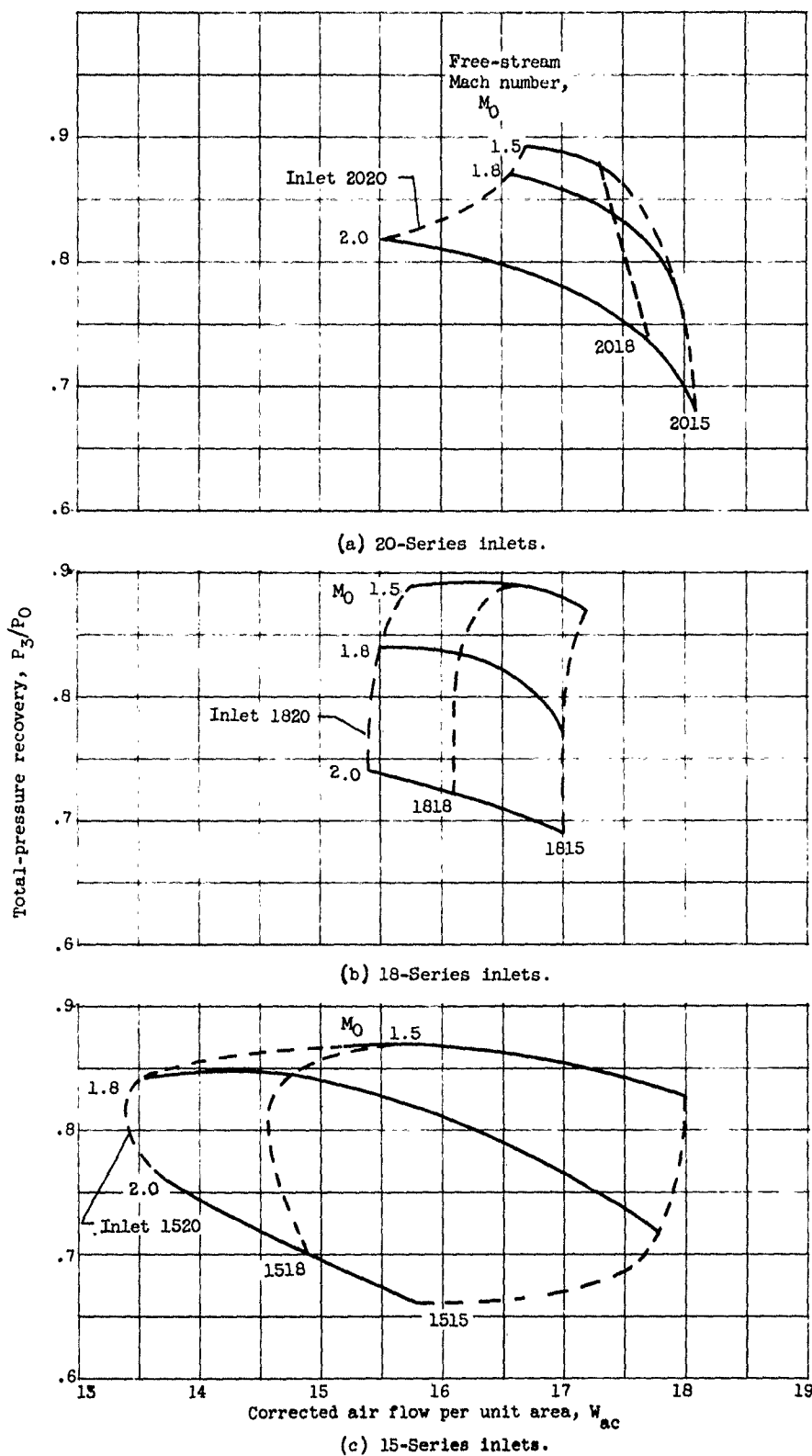
Figure 14. - Corrected air flow maps for critical operation at 9^\circ angle of attack.
