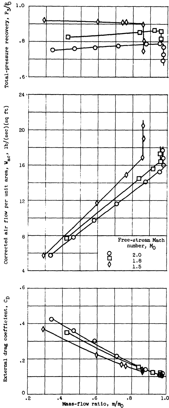
Figure 5. - Continued. Performance of 18-series inlets at zero angle of attack.
