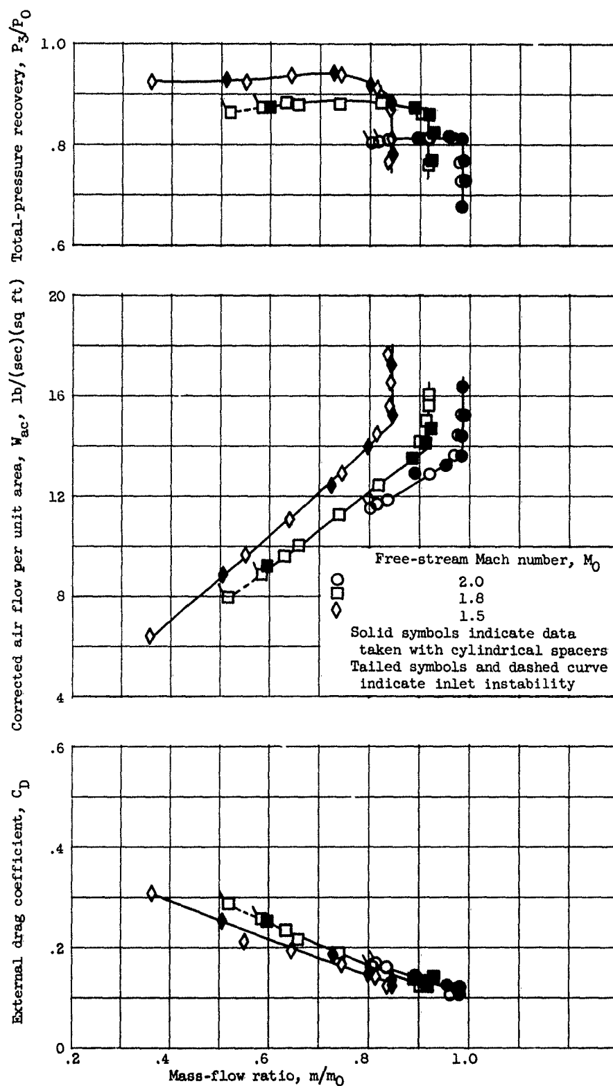
Figure 6. - Performance of 15-series inlets at zero angle of attack.
