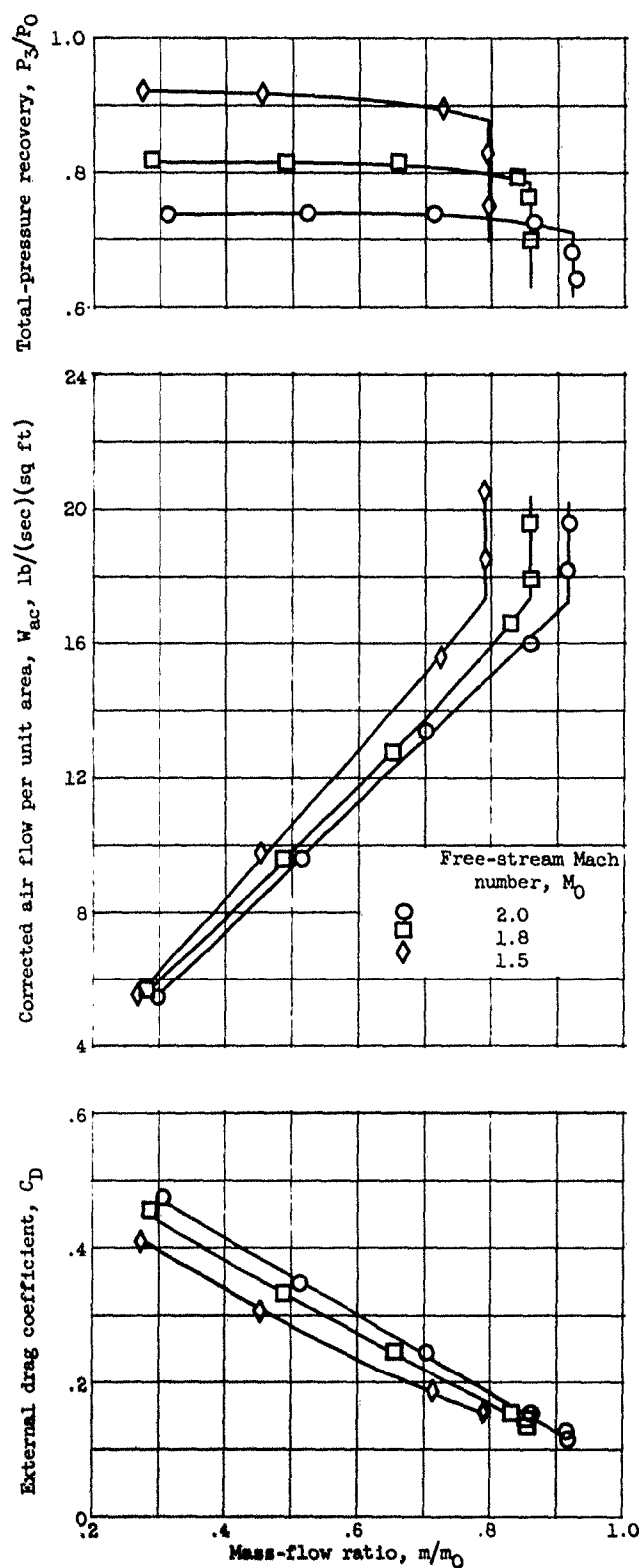
Figure 4. - Concluded. Performance of 20-series inlets at zero angle of attack.
