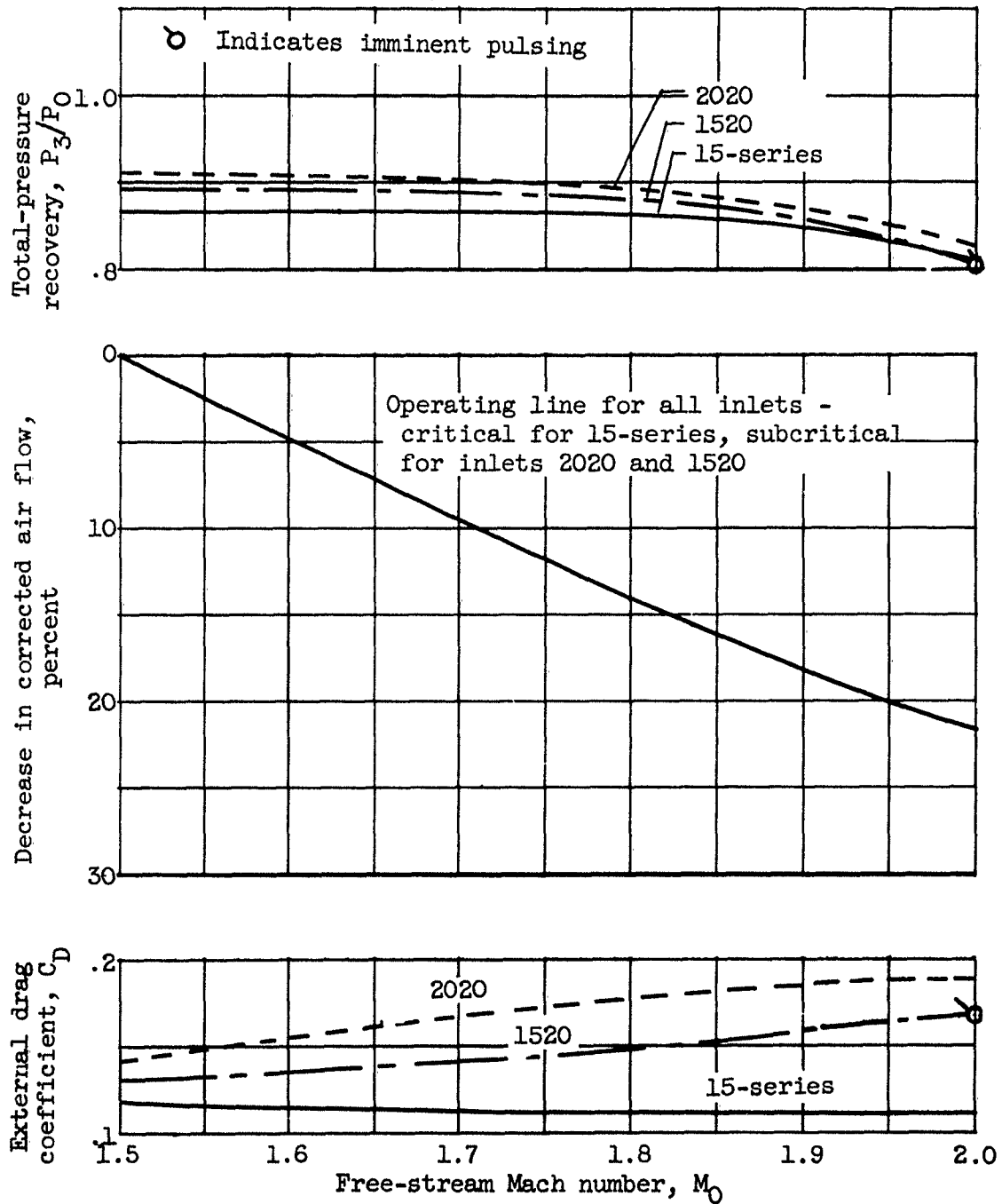
Figure 15. - Performance comparison of fixed-geometry inlets with translating-cone inlet at zero angle of attack.
