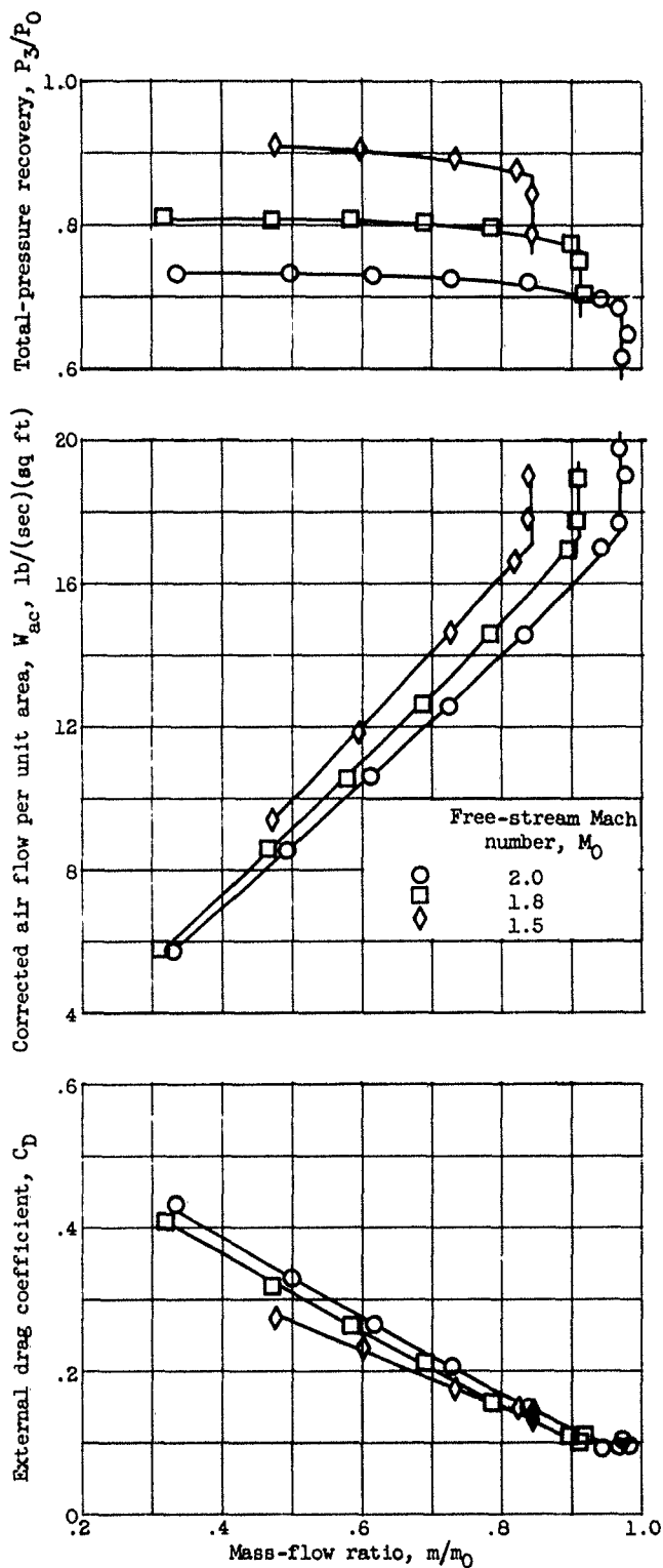
Figure 5. - Concluded. Performance of 18-series inlets at zero angle of attack.
