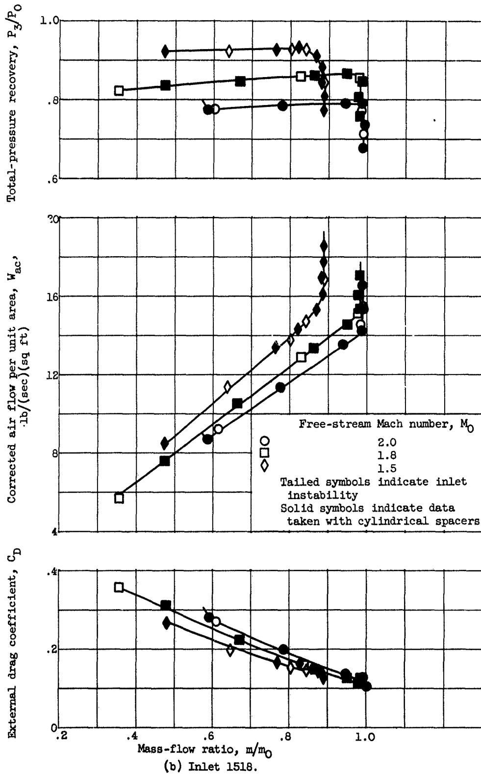
Figure 6. - Continued. Performance of 15-series inlets at zero angle of attack.
