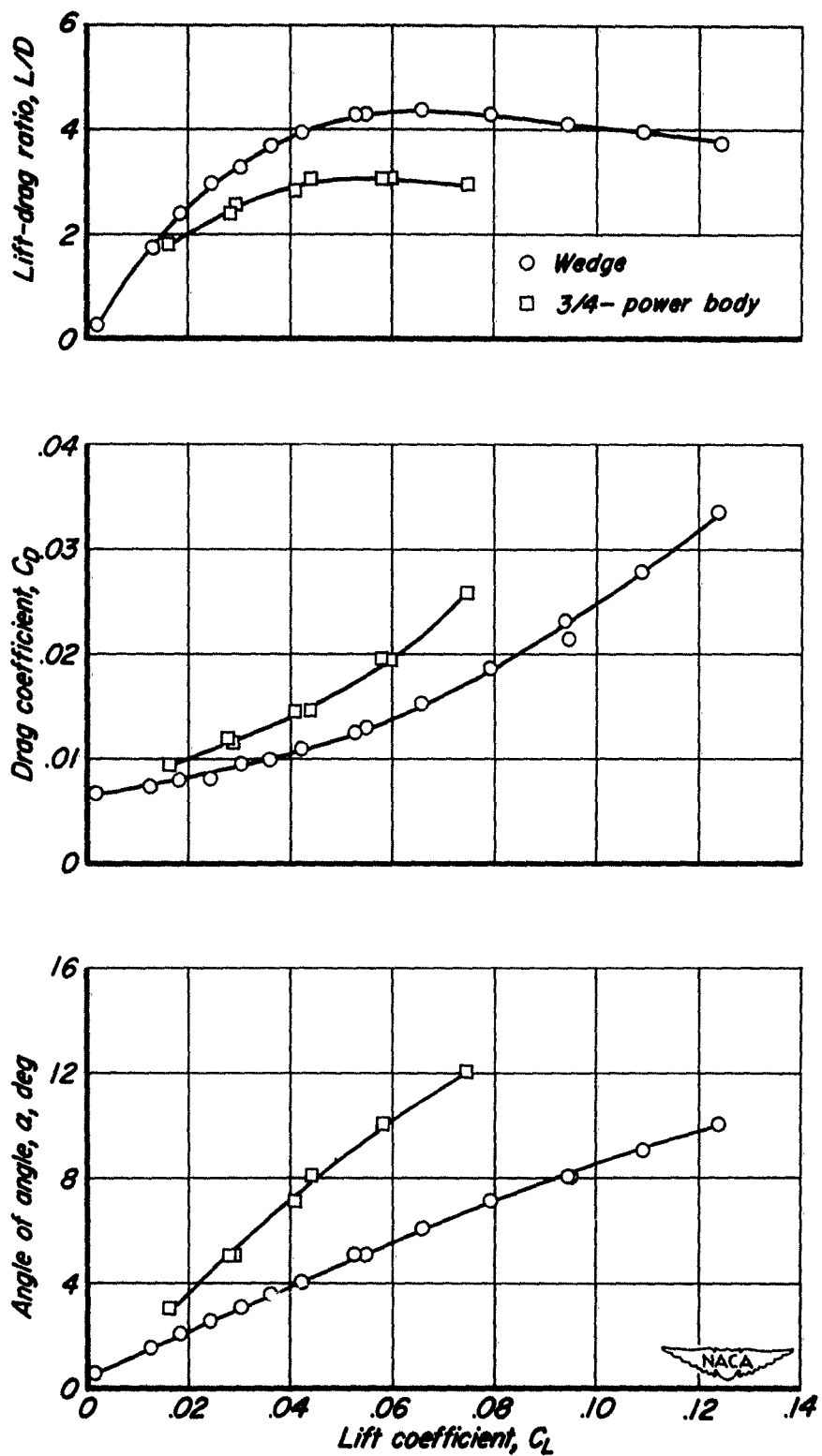
Figure 3.— Comparison of lift-drag curves, drag curves, and lift curves of bodies with fineness ratio 5.
