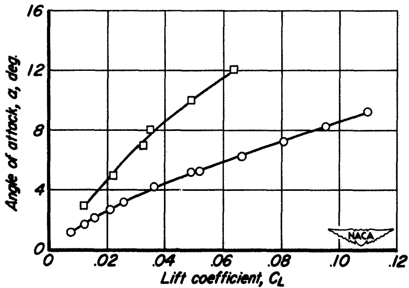
Figure 2.- Comparison of lift-drag curves, drag curves, and lift curves of bodies with fineness ratio 7.
