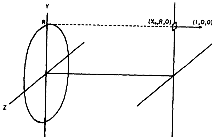
FIG. 3 HILLEBRAND'S PROBLEM
