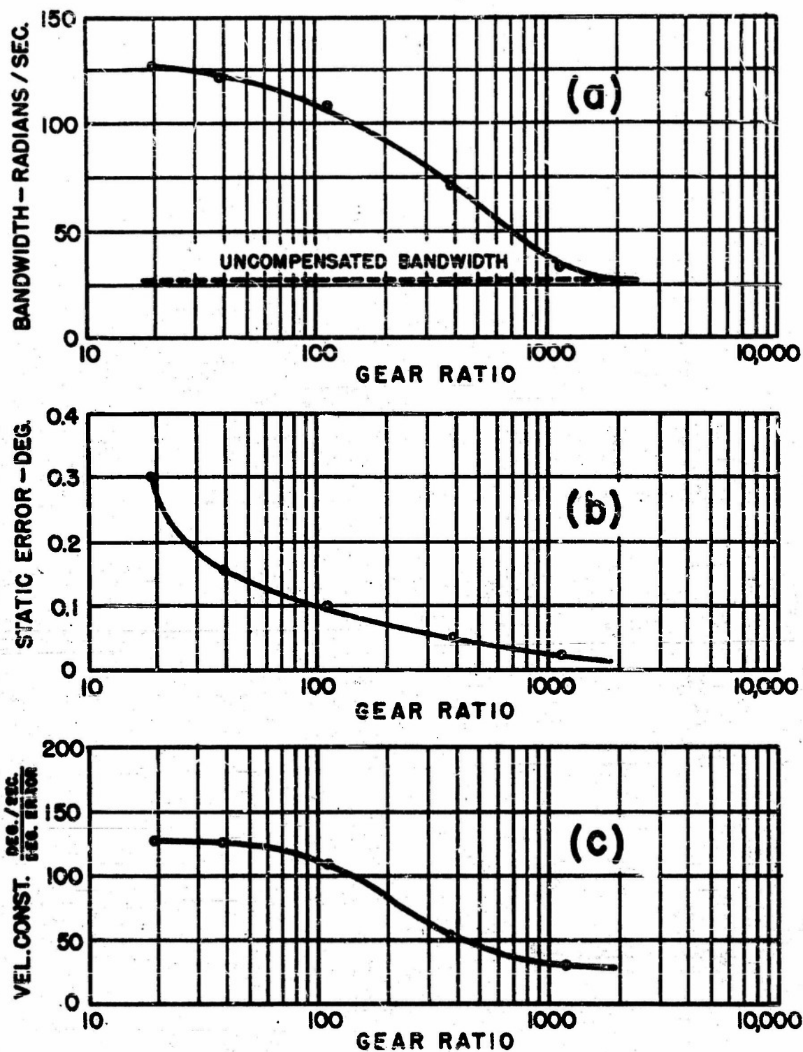
FIG. 13 - SYSTEM PERFORMANCE WITH MARK 7 MOTOR AND NO ADDED INERTIA
