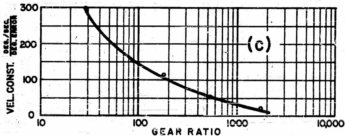
FIG.24- SYSTEM PERFORMANCE WITH MARK 14 MOTOR AND NO ADDED INERTIA
