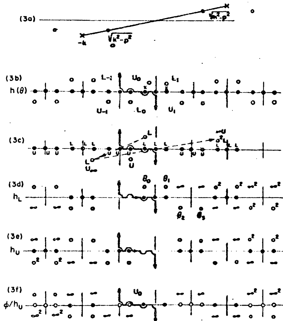
Figure 3 - Contours and singularities for parallel-plate diffraction
