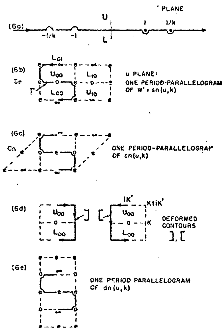
Figure 6 - Contours and singularities for the two-medium diffraction problem.
