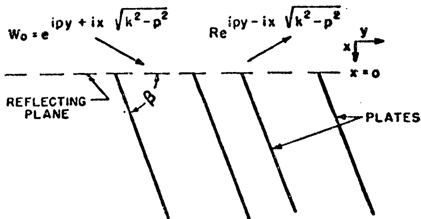
Figure 2 - Parallel-plate surface
