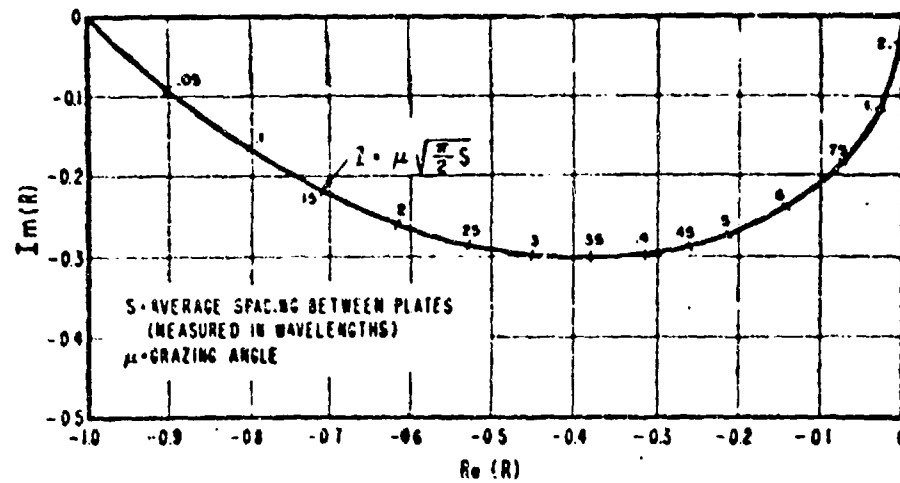
Figure 4 - Complex reflection coefficient, R , of the parallel-plate medium for large average spacing and nearby grazing incidence
