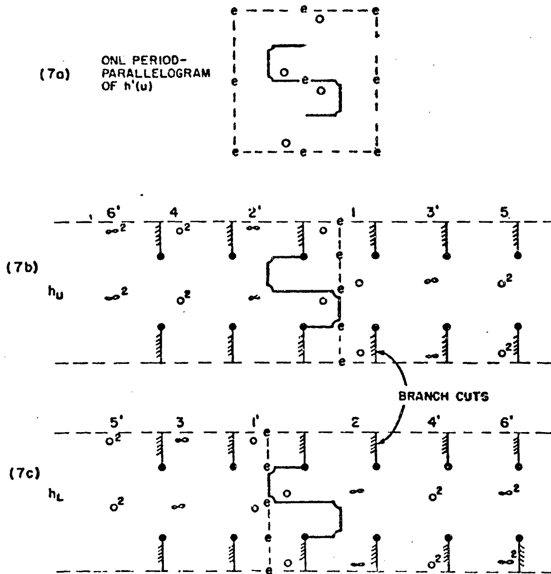
Figure 7 - Structure of h , h_U , and h_L
