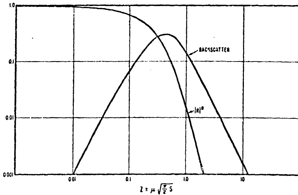
Figure 5 - Specularly reflected and back-scattered power from parallel-plate medium
