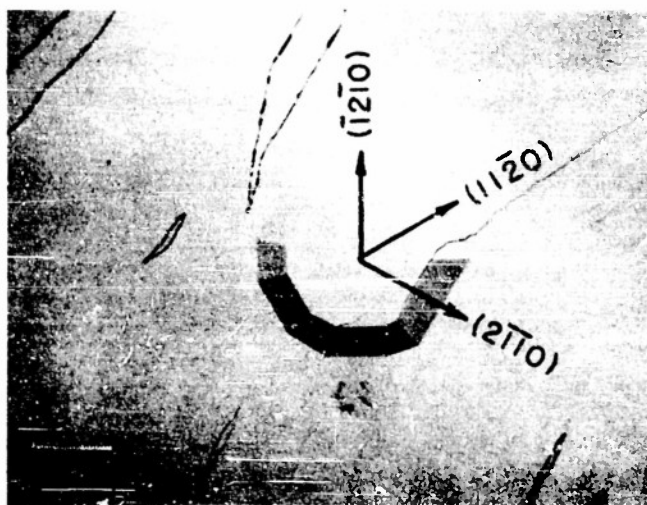
FIG. 20 FINAL STAGE IN THE DISAPPEARANCE OF AN INDENTATION DURING ANNEALING. THE MOST STABLE BOUNDARIES ARE THOSE AT RIGHT ANGLES TO [2\bar{1}10] DIRECTIONS.
