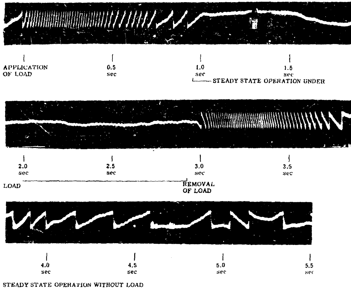
Fig. 25 - Oscilloscope presentation
