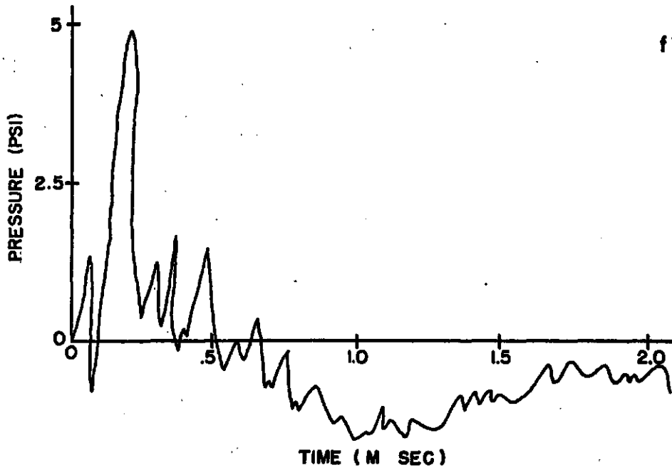
FIG 3 (d thru f) PRESSURE-TIME RECORDS OF A DIFFRACTED SHOCK
