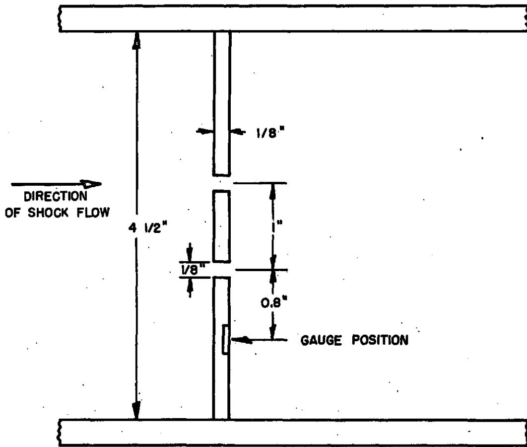
FIG. 1 SKETCH OF GAUGE LOCATION AND WALL DIMENSIONS
