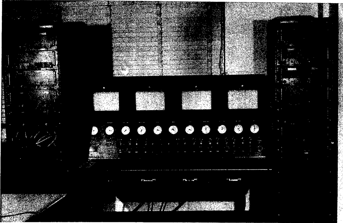
Figure 3: Scoring and Recording Console for Special C-8 Link Trainer
