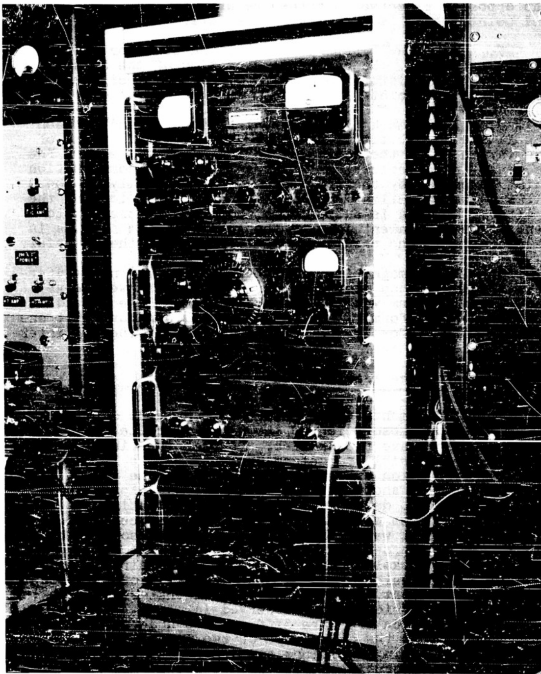
FIG. 2 VARIAN MAGNETIC FIELD METER
