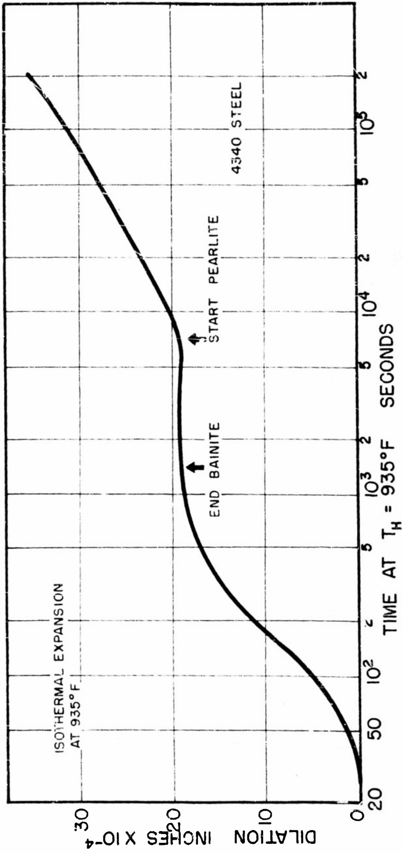
FIG. 18: EFFECT OF TIME AT 935^\circ\text{F} ON AMOUNT OF AUSTENITE TRANSFORMED AT 800^\circ\text{F} .
