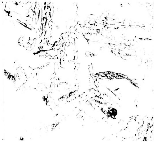
FIG. II: STRUCTURE OF 4340 PRODUCED BY REACTION FOR 1 HOUR AT 930°F FOLLOWED BY 3 MINUTES AT 700°F. NITAL ETCH. 1200 X.
