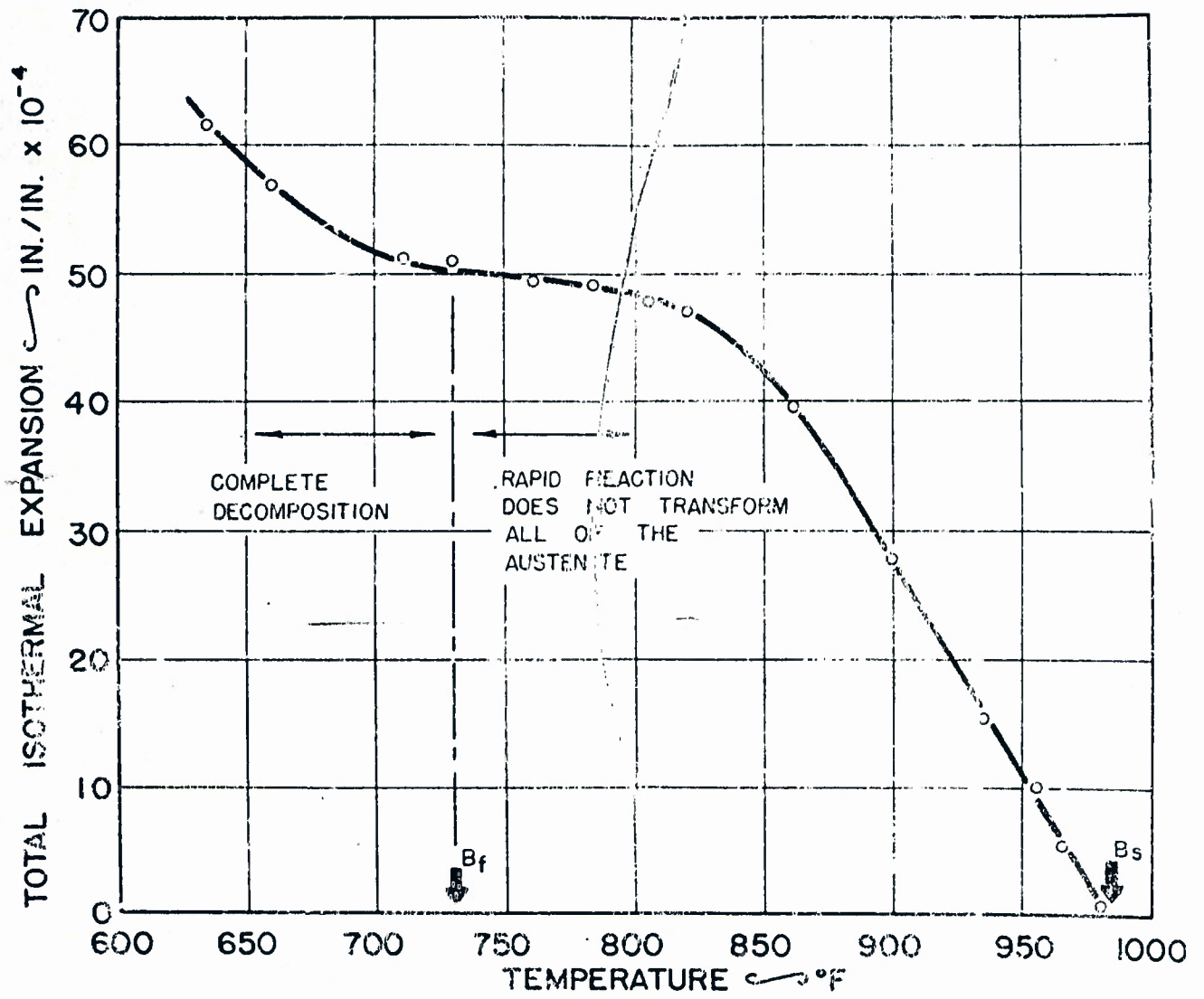
FIG. 4: TOTAL EXPANSION VS. TRANSFORMATION TEMPERATURE FOR 4340 STEEL.
