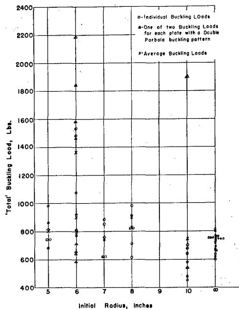
Buckling Loads of .040 Prestressed Flat Plates
