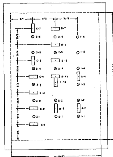
Deflection and Strain Gage Measuring Points on First Series of Aluminum Plates
