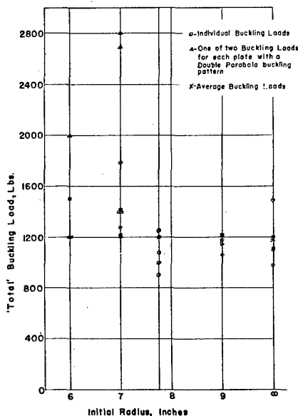
Buckling Loads of .051 Prestressed Flat Plates
