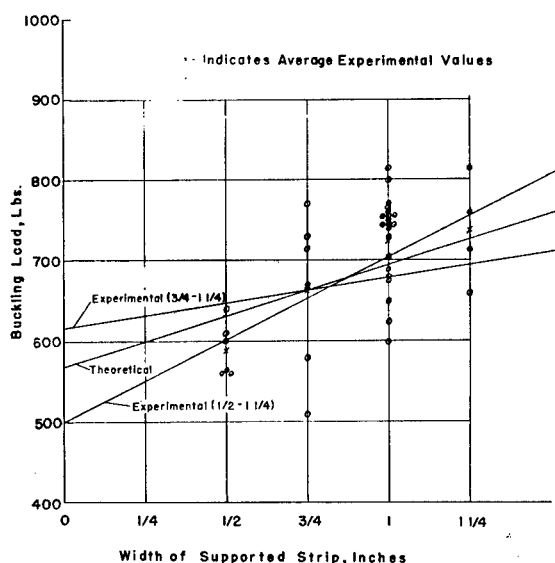
Stringer Calibration Tests (.040 Aluminum Plates)
