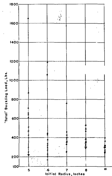
Buckling Loads of .032 Prestressed Flat Plates
