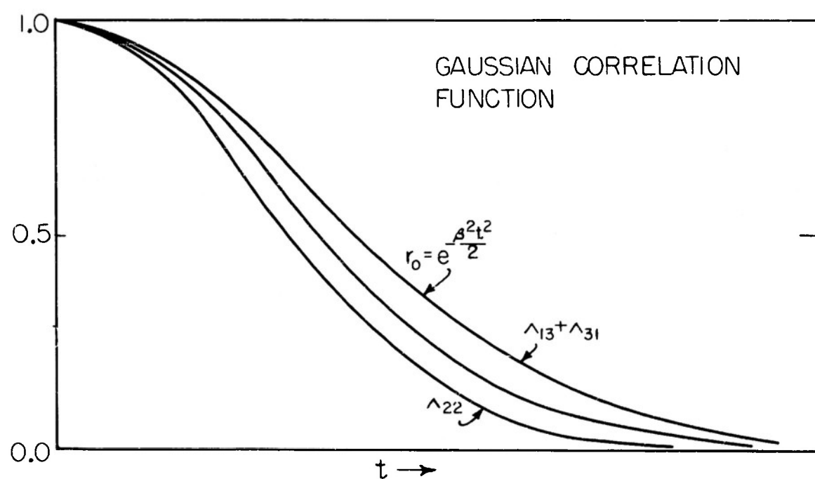
FIG. 6 NORMALIZED SEMI-INVARIANTS
