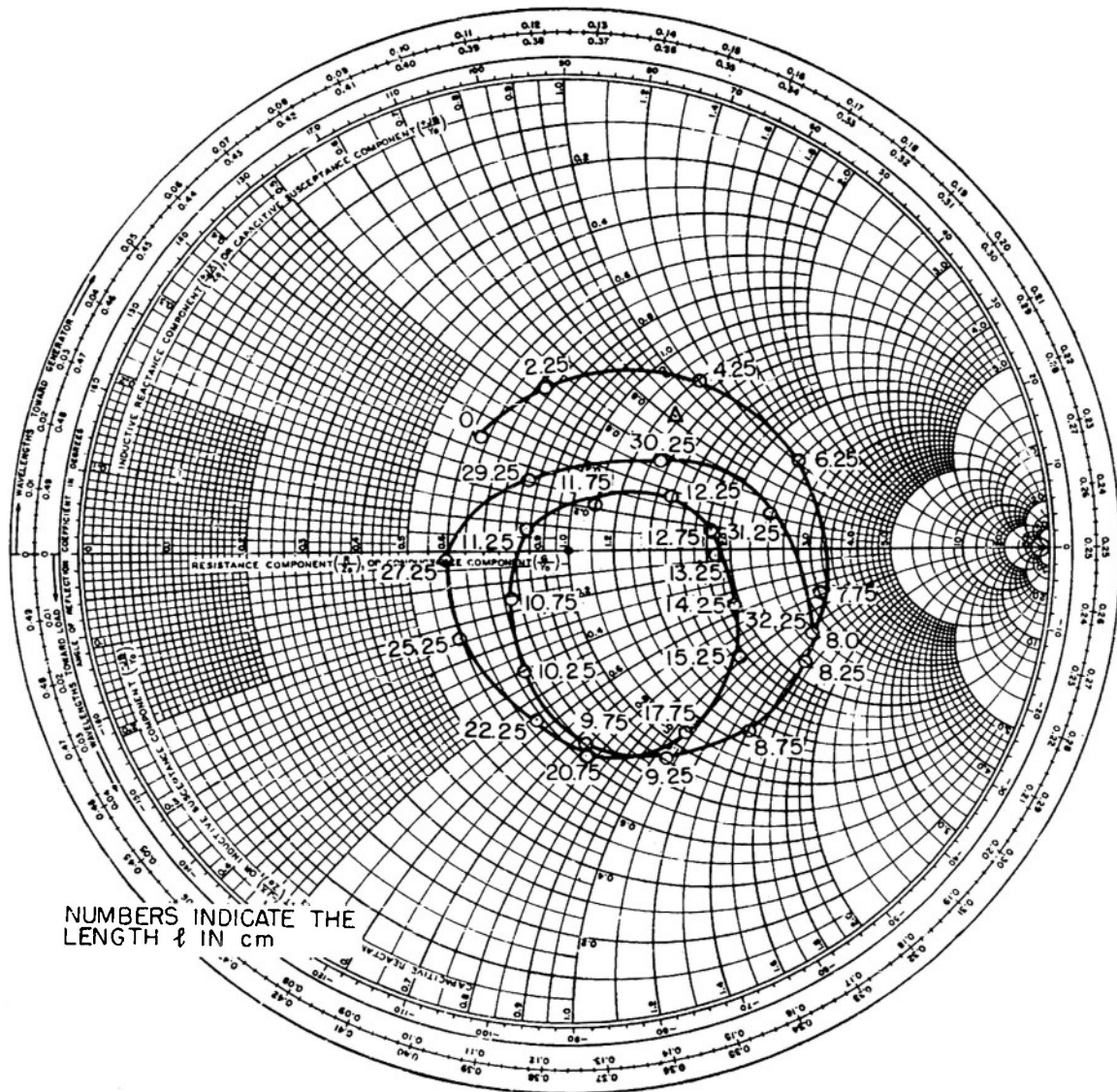
FIG.14 MEASURED IMPEDANCE OF THE COLLINEAR ARRAY WITH TWO-WIRE LINE AS COUPLING ELEMENT
