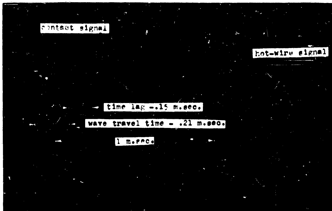
Figure 16. Still Water. Steel Core. Water Impulse Test
