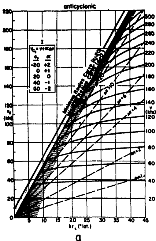
FIG. 6.3: Gradient wind nomograms: (a) anticyclonic, (b) cyclonic [35]. See text for details of computing the gradient wind.
