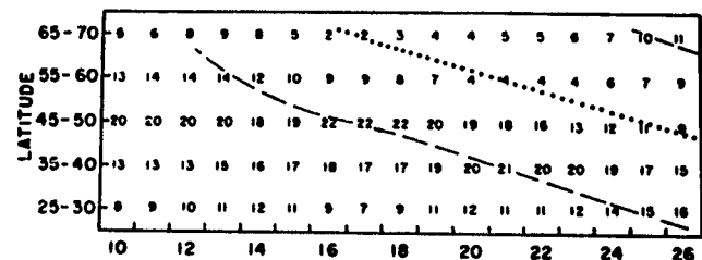
FIG. 5.2: Time section of zonal wind speed (mps) at 500 mb, November 10-26, 1950. Only one quarter of the calculated values is reproduced (every second 5^\circ belt of latitude and every second day). Dashed lines denote relative maxima, and dotted lines relative minima of zonal wind speed [72].
