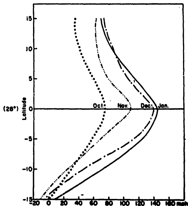
FIG. 3.7: Monthly mean profile of 300-mb zonal wind along 115^{\circ}\text{E} averaged with respect to the center of the southern jet stream computed from fig. 3.6 [112].
