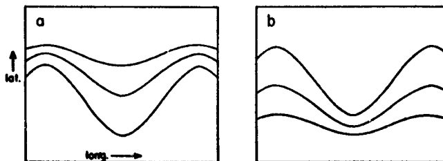
FIG. 5.3: Typical contours of an isobaric surface (a) during Stages NIII and SI, and (b) during stages NI and SIII [72].
