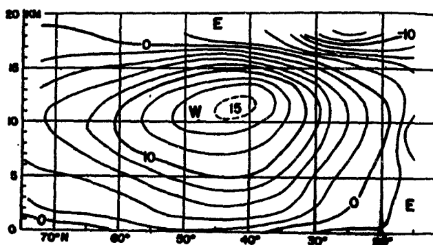
FIG. 3.2b: Same as 3.2a for summer.
