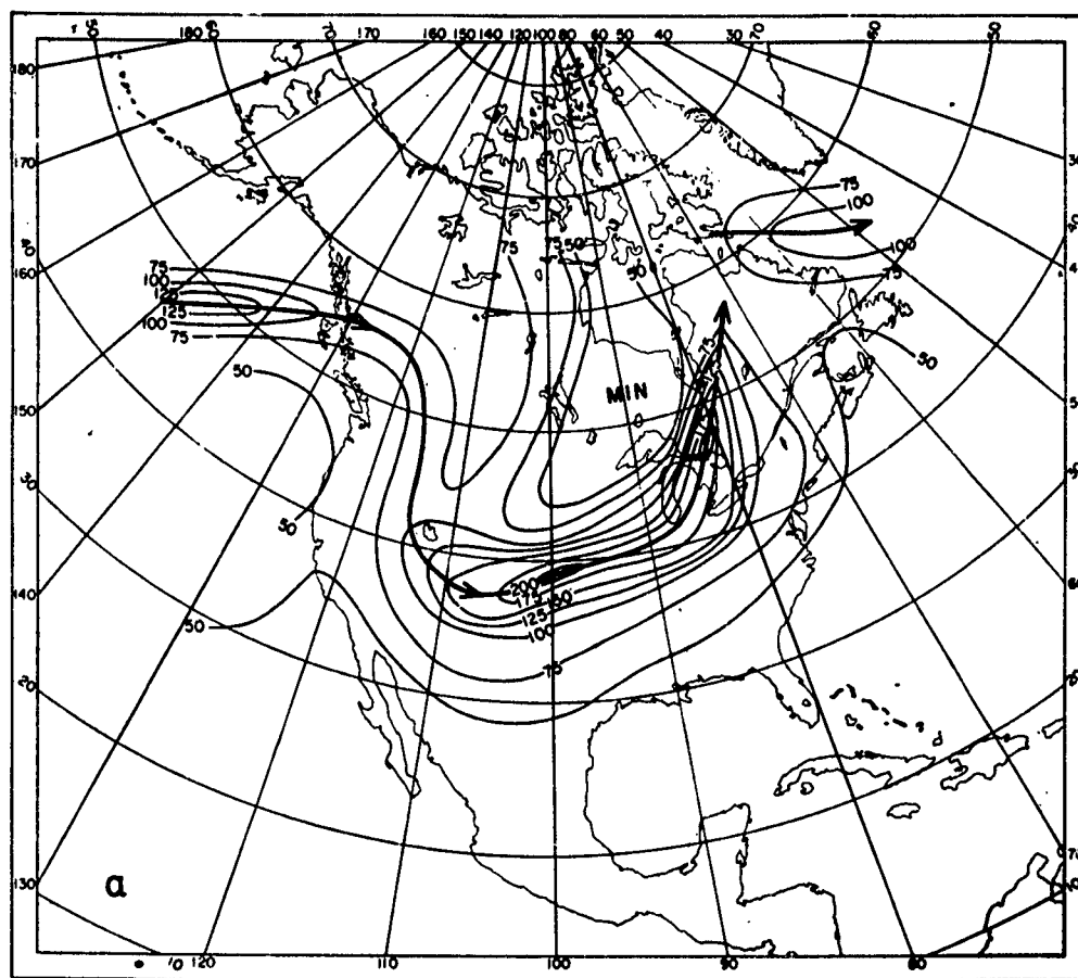
FIG. 2.4a: Isotachs (Knots) at 300 mb, November 10, 1950, 0400 Z. [72].
