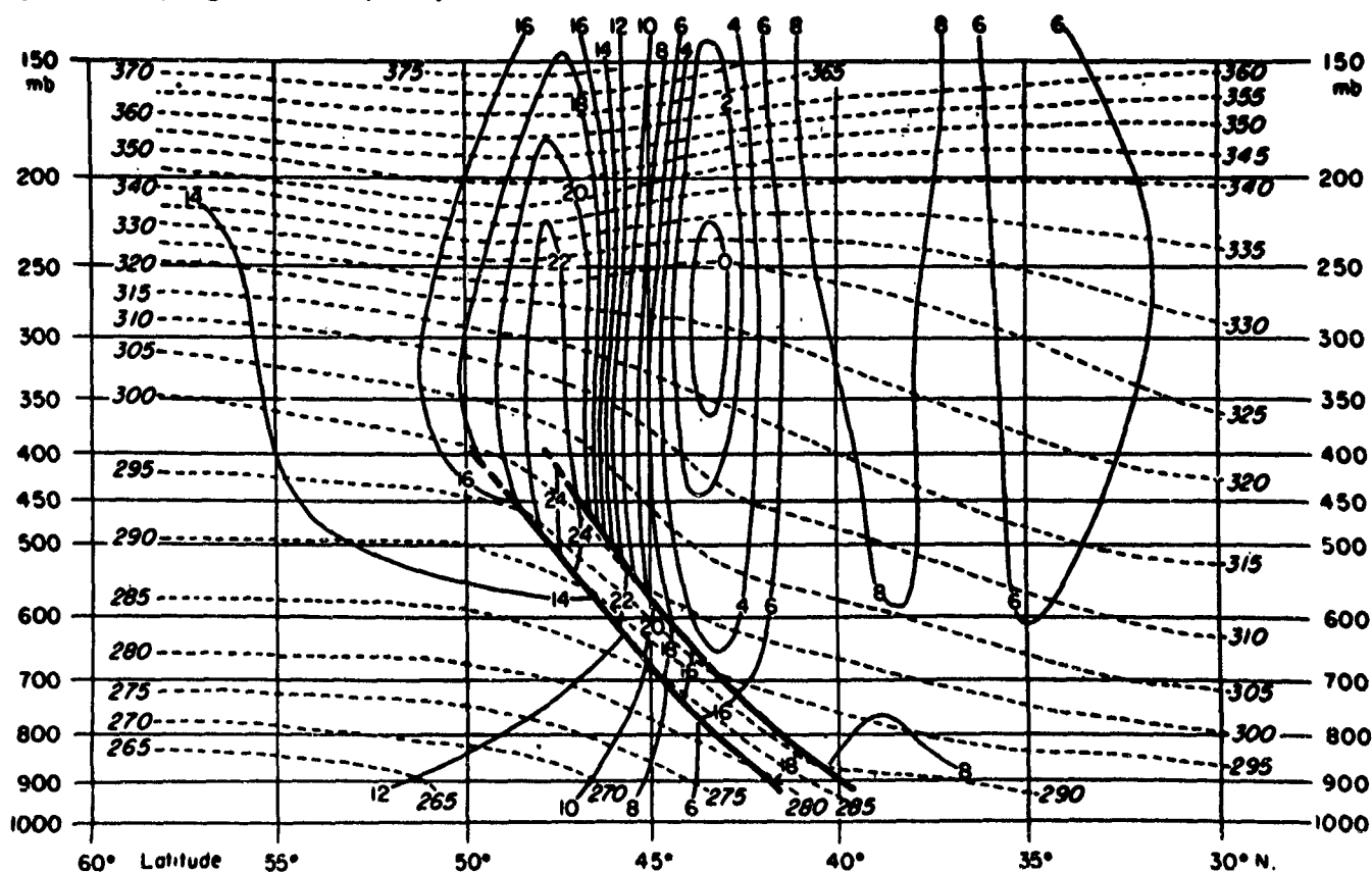
FIG. 2.13: Mean absolute vorticity (solid lines, upright numbers, units 10^{-5} \text{ sec}^{-1} ) and potential temperature (dashed lines, slanting numbers, ^{\circ}\text{A} ) from fig. 2.10. Axis of jet stream corresponds to line 10 \times 10^{-5} \text{ sec}^{-1} vorticity above frontal layer [60].
