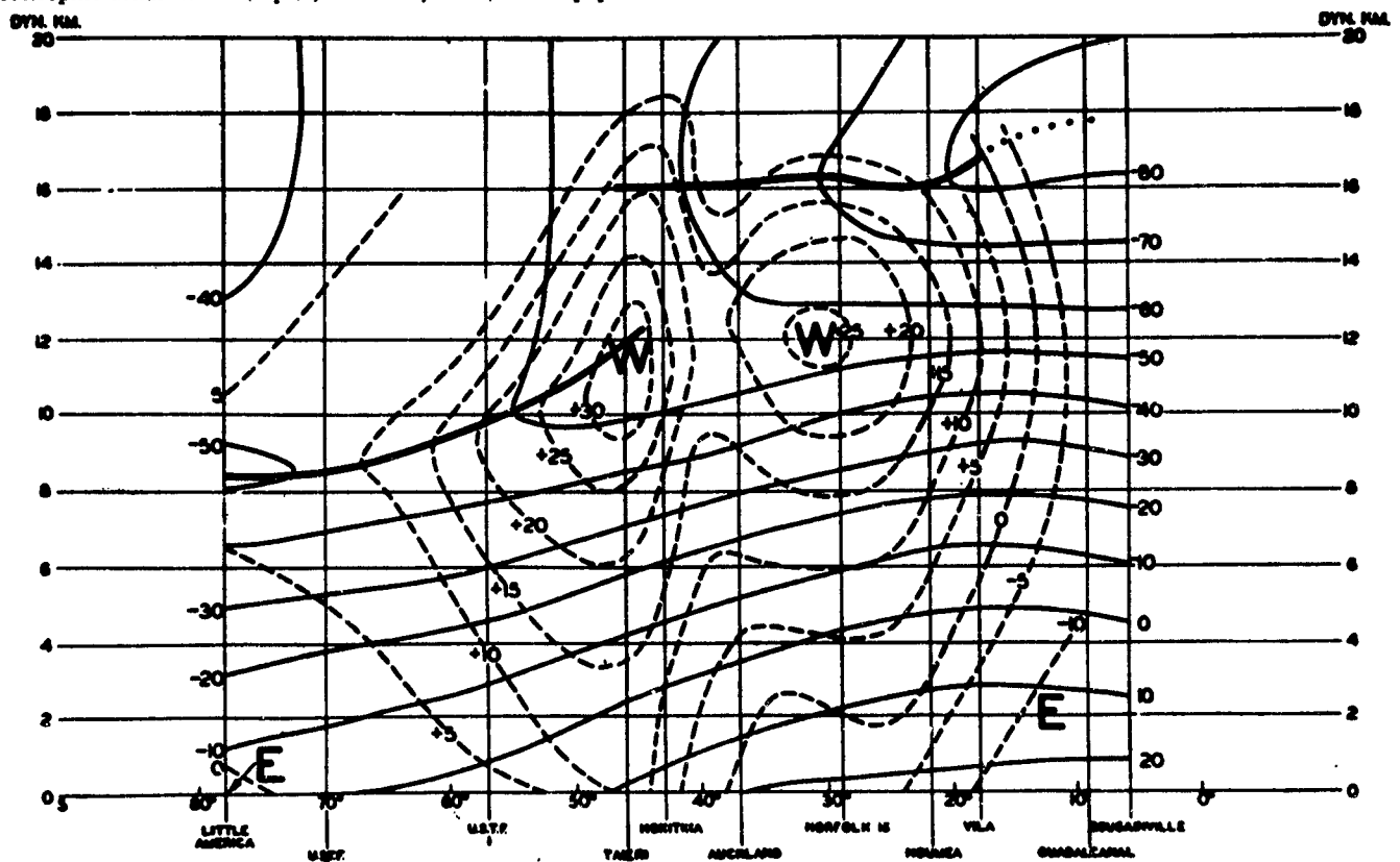
FIG. 3.10a: Meridional cross-section for southern hemisphere winter along 170°E. Thin lines are isotherms ( ^{\circ}\text{C} ); dashed lines, geostrophic zonal winds (mps); and heavy lines, the tropopause [36].
