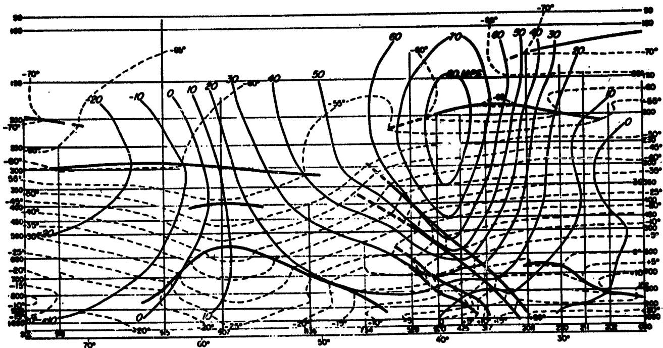
FIG. 2.2: Vertical cross-section approximately along the meridian 80°W from Havana in the south to Thule (Greenland) in the north. Vertical lines indicate the soundings used in the diagram with the international station numbers below. Frontal boundaries, inversions or tropopause surfaces are indicated by thick, solid lines when they are distinct, and by thick, dashed lines when not distinct. Thin solid lines indicate geostrophic wind velocity (mps) perpendicular to the cross-section, dashed lines isotherms (°C) [55].
