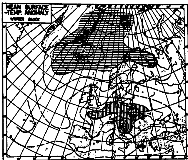
FIG. 3.20: European winter temperature anomalies during blocking. Lines of equal temperature anomaly are given for each 2^{\circ}\text{C} above and below normal and are shown by the thin dashed lines. Areas recording mean temperatures more than 4^{\circ}\text{C} above normal are indicated by the horizontal hatchings and areas recording mean temperatures more than 4^{\circ}\text{C} below normal by the vertical hatchings [67].
