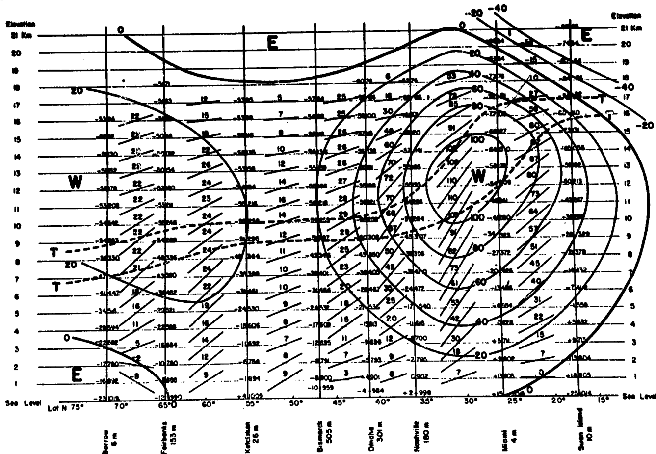
FIG. 1.3: Vertical cross-section of pressure (mb), temperature ( ^\circ\text{C} ) and wind (knots) for North America during winter [108].
