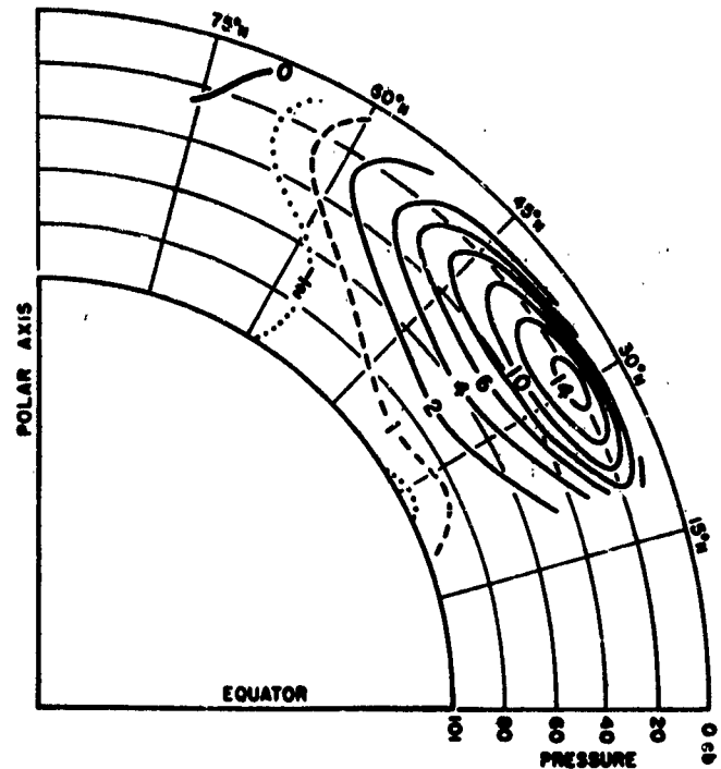
FIG. 7.7: The mean geostrophic poleward flux of angular momentum in 10^{14} \text{ t m}^2 \text{ sec}^{-2} per layer of 10 mb thickness in January 1949 [47].
