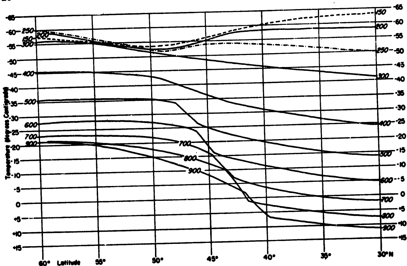
FIG. 2.20: Profiles of temperatures of isobaric surfaces (labelled in slanting numbers) taken from fig. 2.10. The latitudinal temperature gradient at any isobaric level may be judged by the slope of the profile [60].
