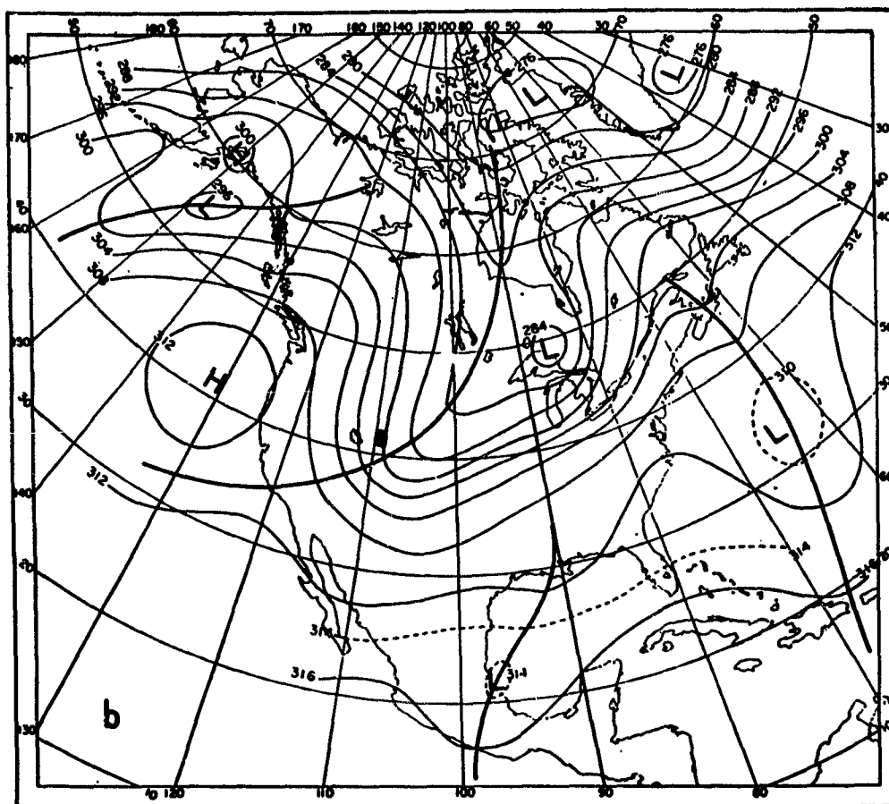
FIG. 2.4b: Contours at 300 mb, November 10, 1950, 0400Z [72].
