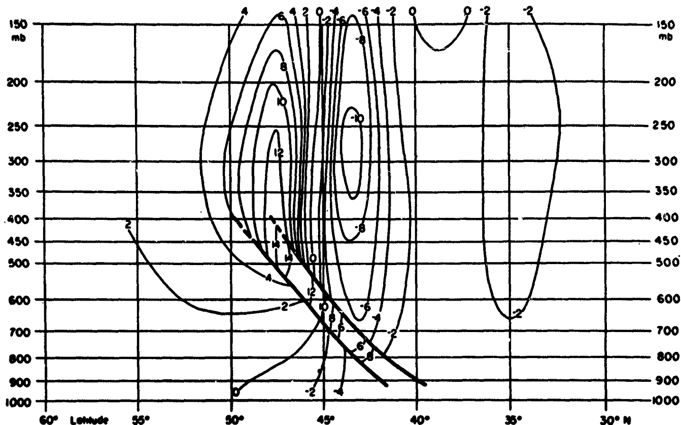
FIG. 2.12: Mean horizontal wind shear from fig. 2.10. Units are \text{m/sec}/(100 \text{ km}) , or 10^{-5} \text{ sec}^{-1} . Positive numbers indicate cyclonic shear; negative numbers, anticyclonic shear [60].
