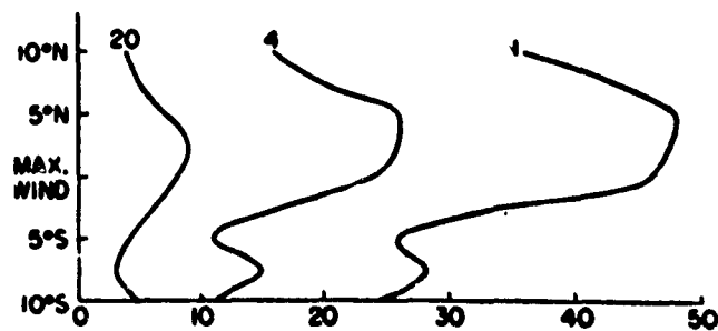
FIG. 3.23: Profiles of frequency (per cent) of precipitation relative to jet streams with troughs, obtained by averaging longitudinally from 20 degrees east to 20 degrees west of troughs. Curves 1, 4, and 20 have same significance as in fig. 3.22 [96].
