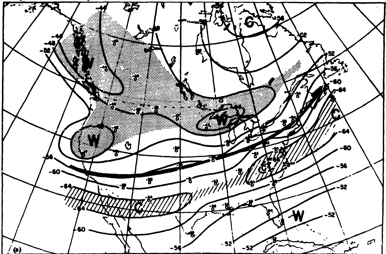
FIG. 2.21: Isotherms ( ^{\circ}\text{C} ) at 200 mb, January 28, 1947, 0300Z. Heavy arrow indicates center of jet [68].
