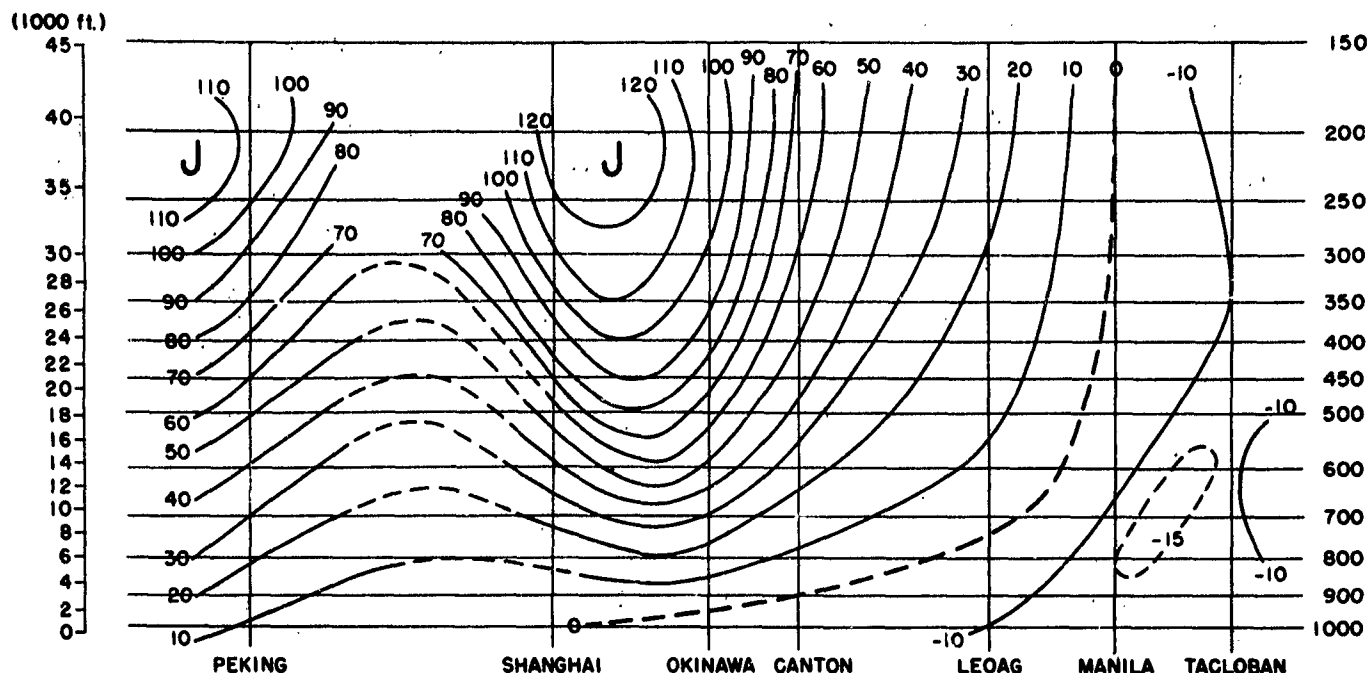
FIG. 3.5: Meridional cross-section of mean zonal wind (mph) for December 1945 and January 1946 computed from rawin data along 120°E [112].
