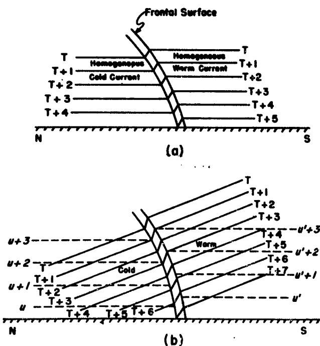
FIG. 1.1: Schematic representation of the wind and temperature fields in the vicinity of a frontal surface according to classical concepts: (a) level isotherms and a uniform current in each air mass; (b) sloping isotherms and currents ( u, u' ) increasing uniformly with height.
