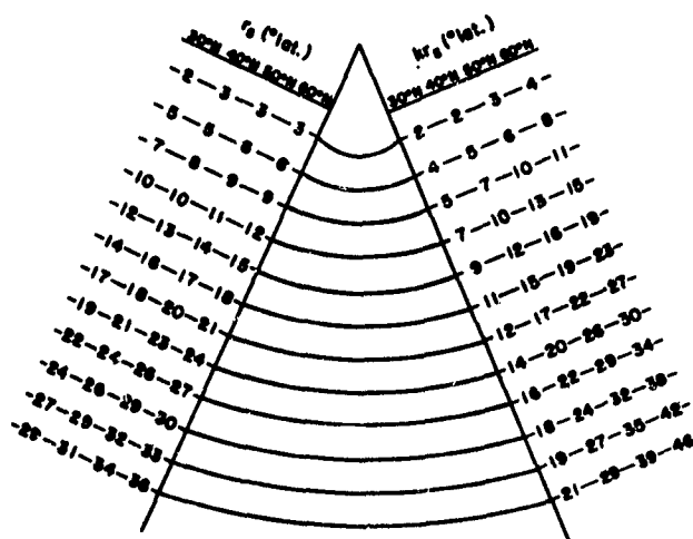
FIG. 6.2: Overlay for measuring radius of streamline curvature on polar stereographic projection, true at lat. 60°. Numbers on left give radius of curvature, r_s , in °lat. at indicated latitudes; numbers on right give r_s multiplied by latitude factor, k .
