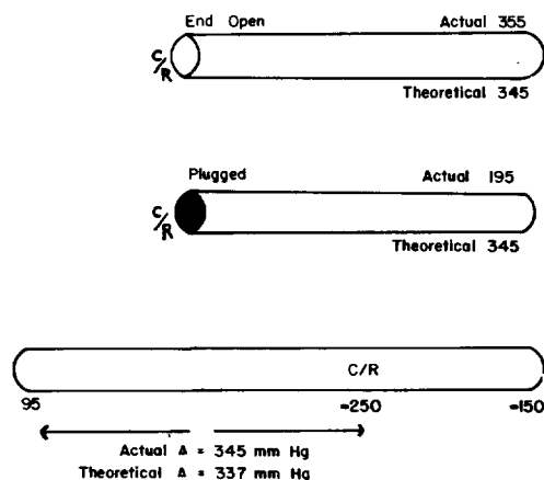
Figure 16 - Behavior of model systems during tumbling. C/R is point at which center of rotation was located in each case.
