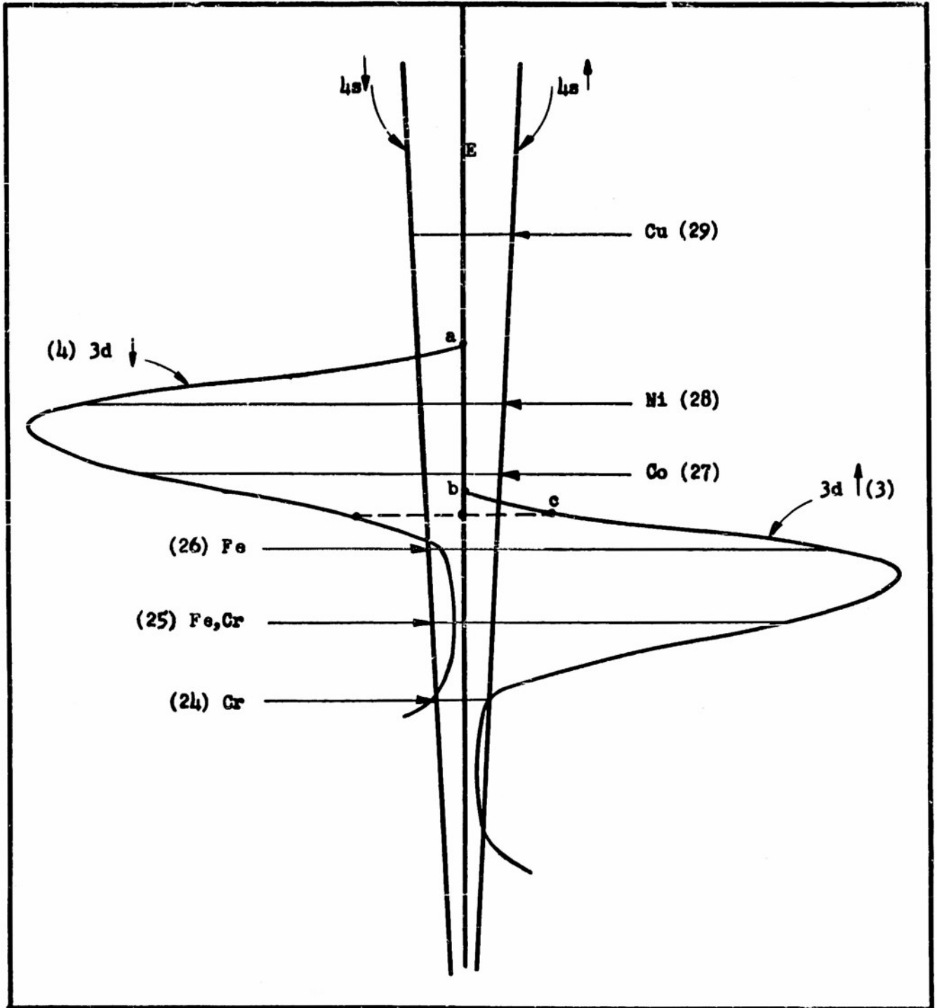
Fig. 5 Assumed density of states versus energy curves for the two 4s and the two 3d bands used in analyzing the data. The bands with spins parallel to the field are plotted to the right while those with antiparallel spins are plotted to the left of the energy axis.
