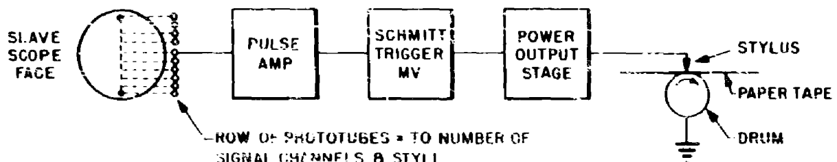
Figure 31 - Block diagram of Model I system
