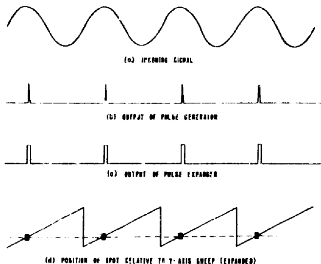
Figure 4 - Graphic Indicator waveforms
