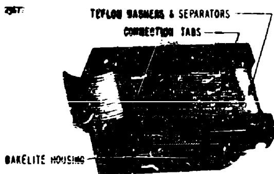
Figure 28 - Stylus head assembly (bottom view)
