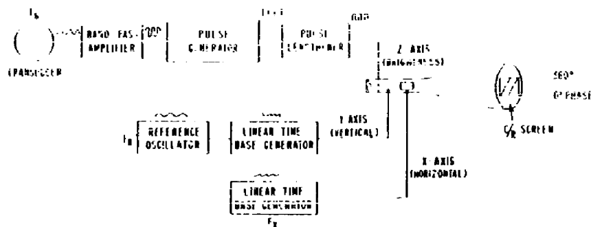
Figure 3 - Sonar Graphic Indicator (simplified)
