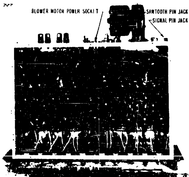
Figure 14 - Coincidence unit (bottom view)
