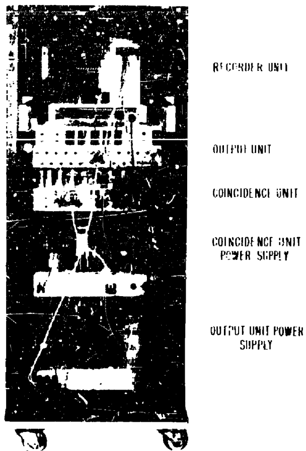
Figure 10 - Phase recorder assembly (rear view)
