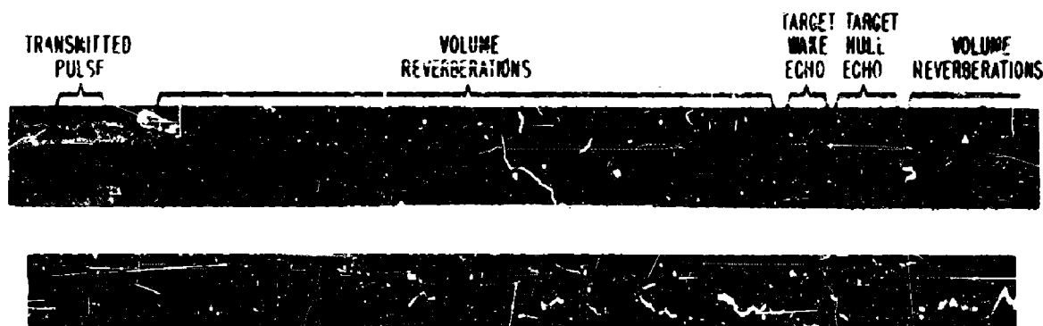
(b) Reference frequency oscillator set to average reverberation echo frequency
