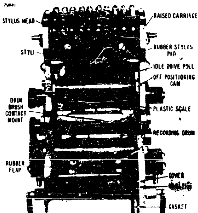
Figure 48 Stylus-type recording head, Models I and II
