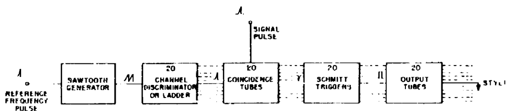
Figure 11 - Block diagram of phase recording system
