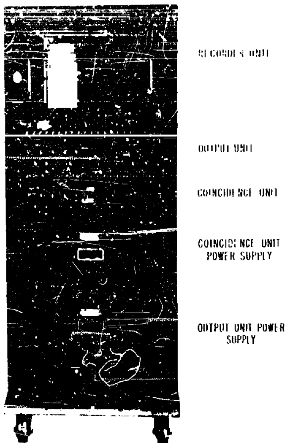
Figure 9 - Phase recorder assembly (front view)
