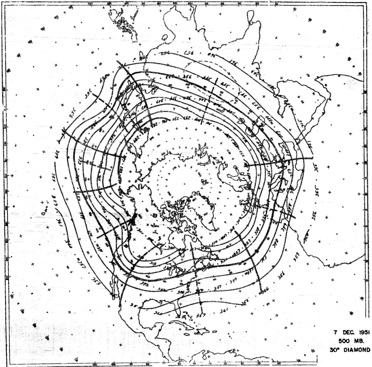
Figure (1k). Space Mean - 30° Diamond - 7 December 1951
