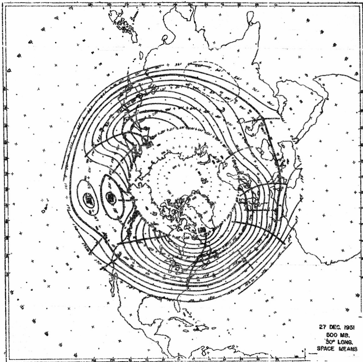
Figure (2f). Space Mean - 30° Longitude - 27 December 1951
