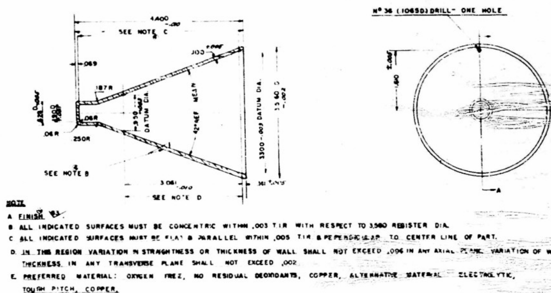
Fig. 4. DRB398 Conical Liner. From Which DRD393 Liners Were Pressed.
