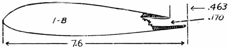
PRINCETON T.E. SLOT MODEL 1-B
