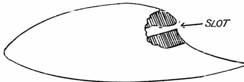
BRITISH 31.5% THICK SLOTTED AIRFOIL
