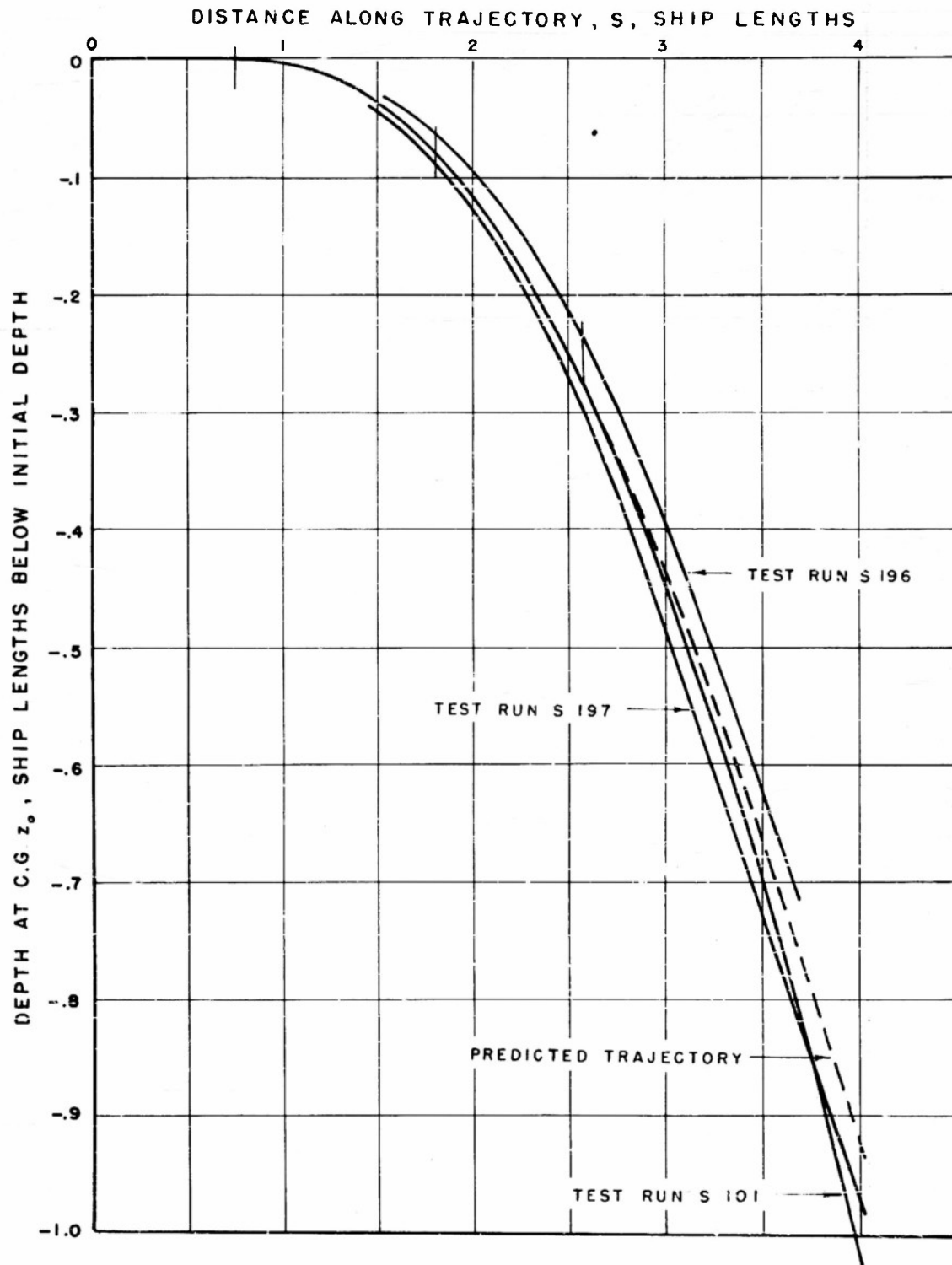
Fig. 5 - Depth curves.
