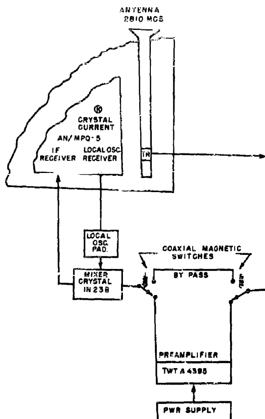
Fig. 1 - Modification of AN/MPQ-5 radar for traveling-wave tube preamplifier addition
