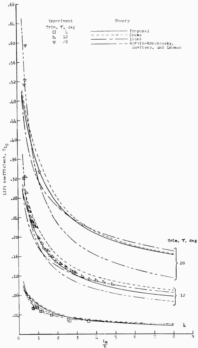
(a) Trim of 4°, 12°, and 20°.
