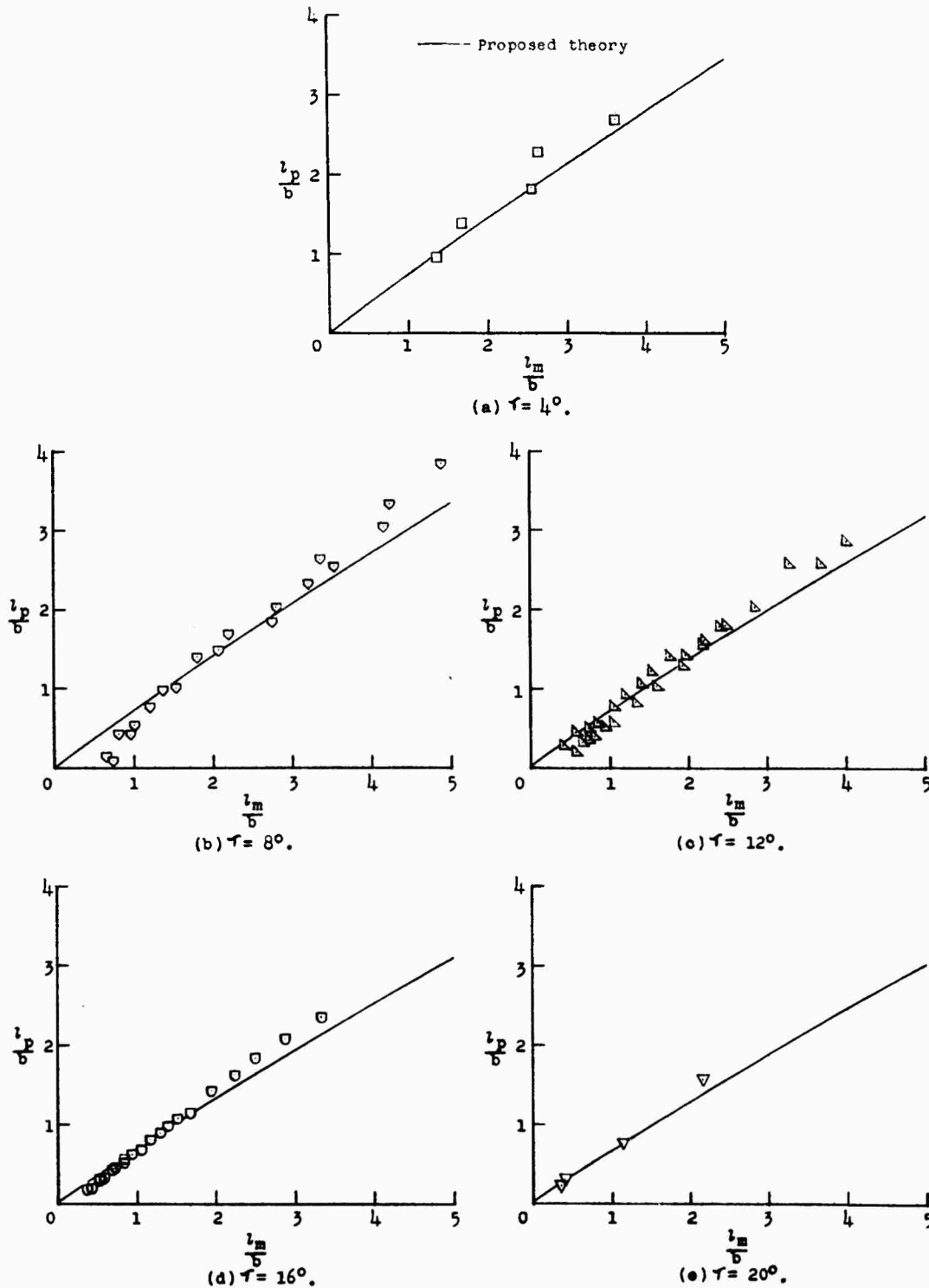
Figure 12.- Variation of center-of-pressure ratio with mean wetted-length-beam ratio for a 2.5-inch-beam rectangular-flat-plate planing surface (unpublished NACA data).
