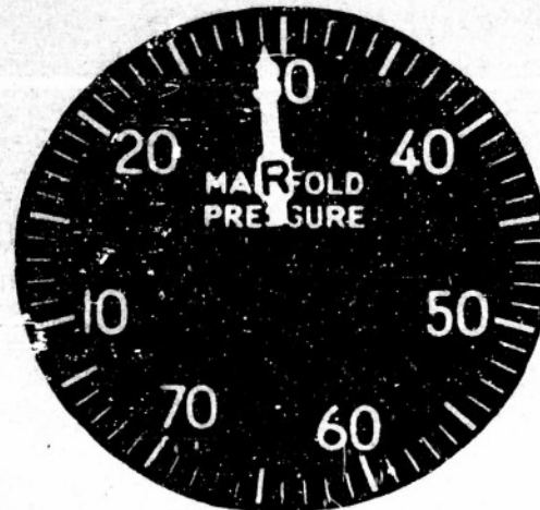
Type 2 Dial 4% error
