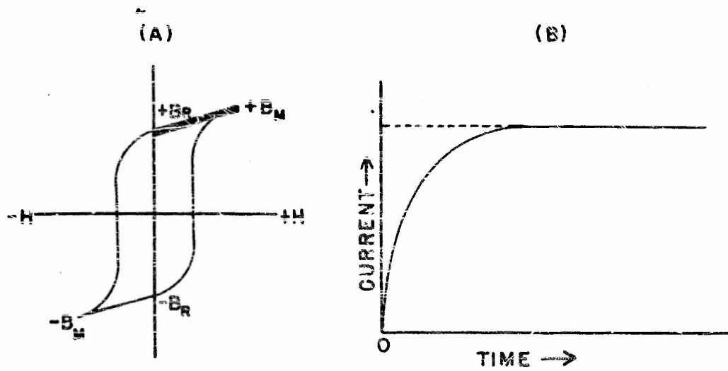
FIG. 4. CURRENT vs. TIME AS FLUX CHANGES FROM +B_R TO +B_M
