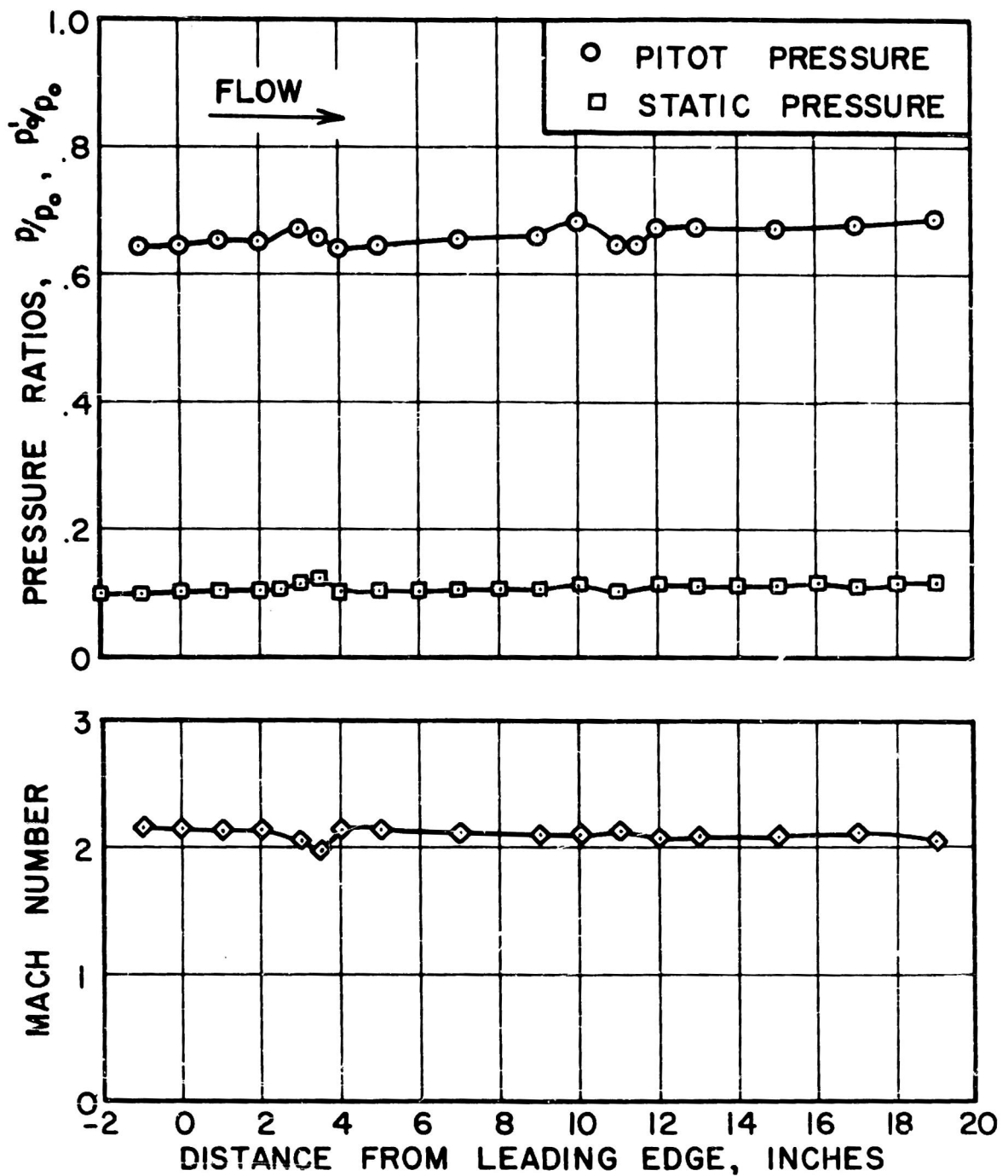
FIG. 14 PRESSURE AND MACH NUMBER DISTRIBUTION ALONG CENTERLINE OF HOLLOW CYLINDER WITH 10^\circ EXTERNAL BEVEL AND BOW SHOCK "SWALLOWED", M = 2.15
