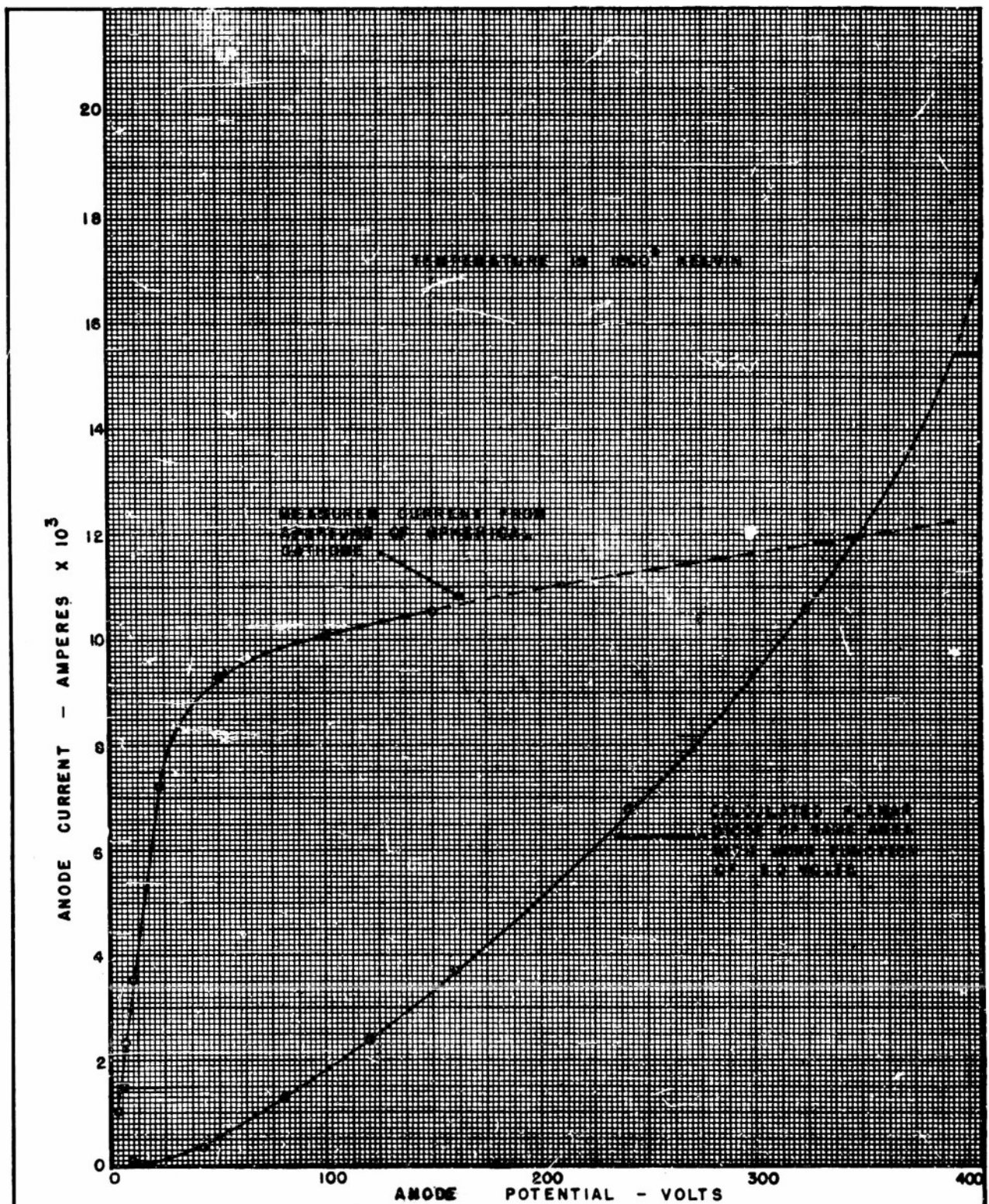
FIGURE 3 COMPARISON OF SPHERICAL CATHODE APERTURE CHARACTERISTIC AND CALCULATED PLANAR DODE CHARACTERISTIC
