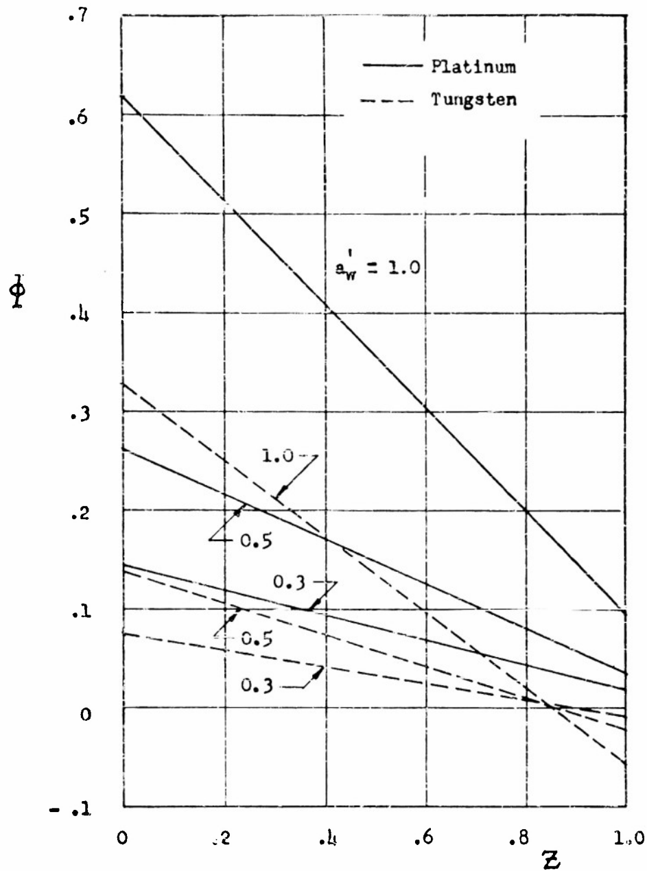
Figure 39.- Hot-wire \Phi correction based upon equation (22).
