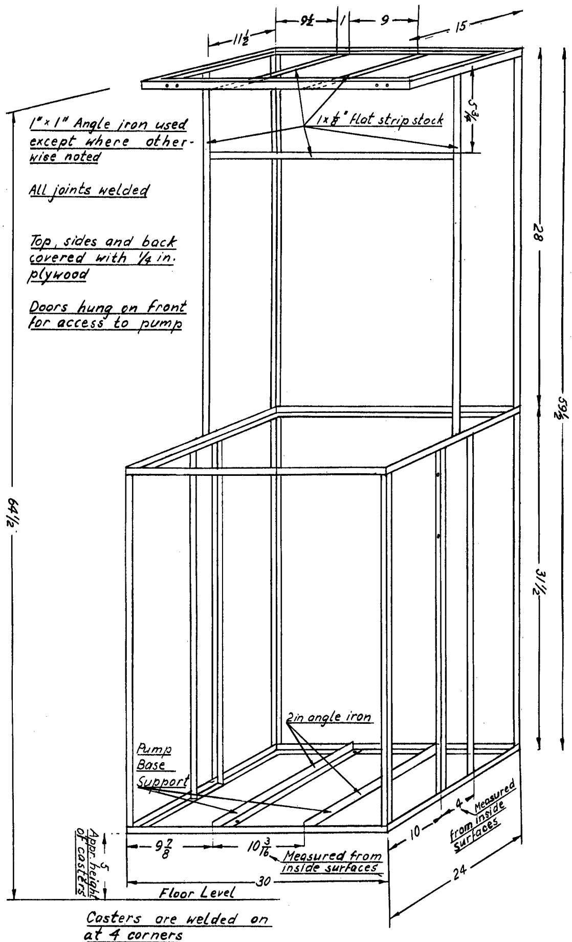
Figure 17. Portable Leak Meter Frame
