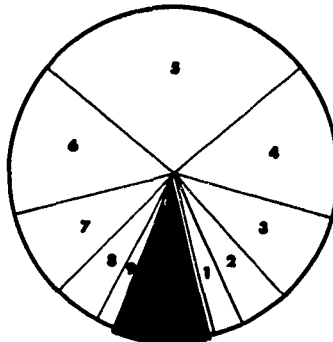
Fig. 3B EQUIVALENT NUMBER OF EQUIPROBABLE ALTERNATIVES \approx 8 H = 3.01
