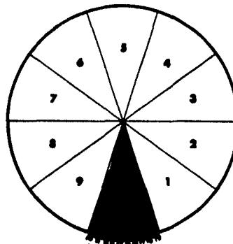
Fig. 2B 9 MAJOR, 10 MINOR ALTERNATIVES Equivalent number of equiprobable alternatives: 13 H = 3.63
