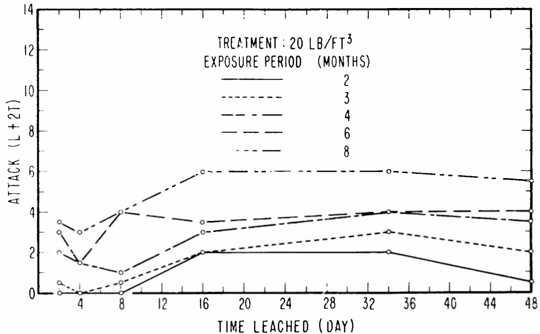
Figure 7 - Relation between attack and leaching time for whole creosote treatments for various exposure periods
