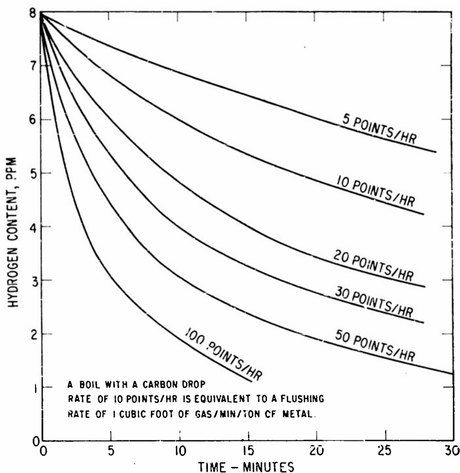
Fig. 9 — Theoretical flushing curves showing effect of carbon boil rate on the hydrogen content of liquid iron.
