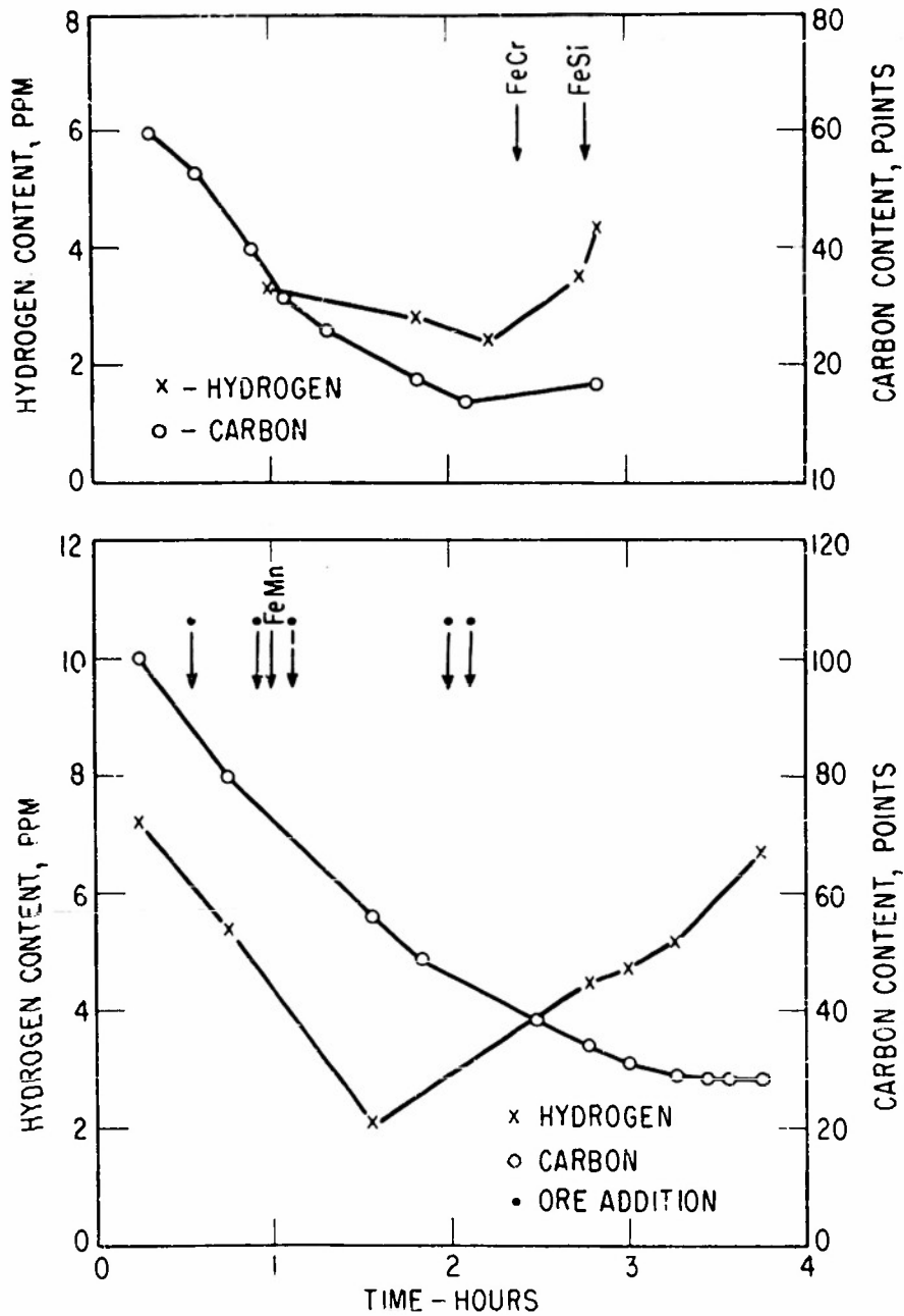
Fig. 6 — Typical hydrogen and carbon heat logs for acid open hearth steels. (Top log from authors' work; bottom log from Wentrup, et al 12 )
