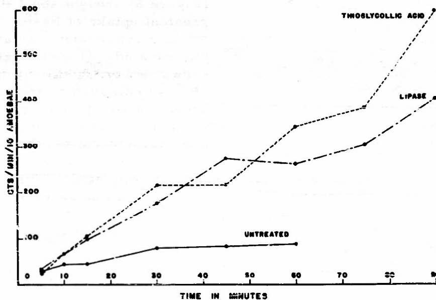
Figure 9. Radioactivity of Amoebae untreated and treated with lipase and thioglycollic acid.
