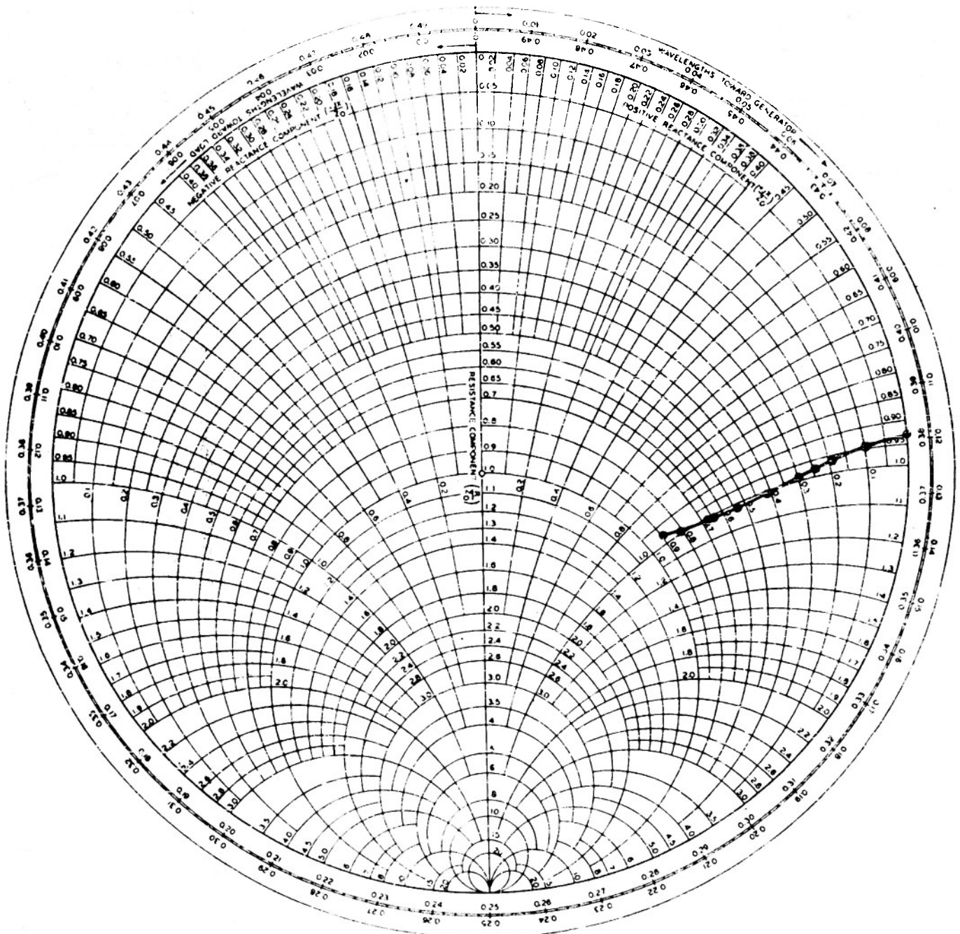
FIG. 8 INPUT IMPEDANCE FOR DELAY LINE OSCILLATOR PLOTTED IN A SMITH CHART
