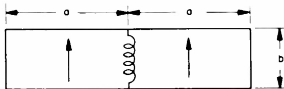
FIGURE 1 TRANSVAR DIRECTIONAL COUPLER, CUTAWAY VIEW
