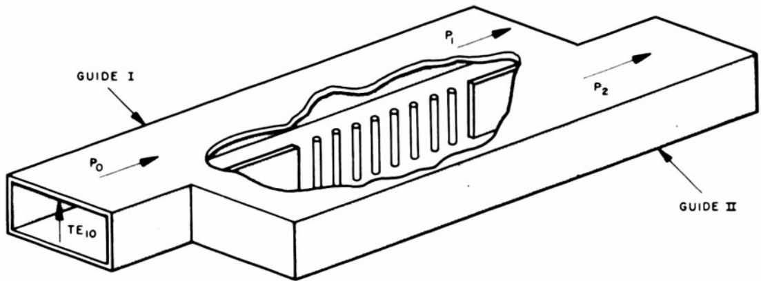
FIGURE 1 TRANSVAR DIRECTIONAL COUPLER, CUTAWAY VIEW
