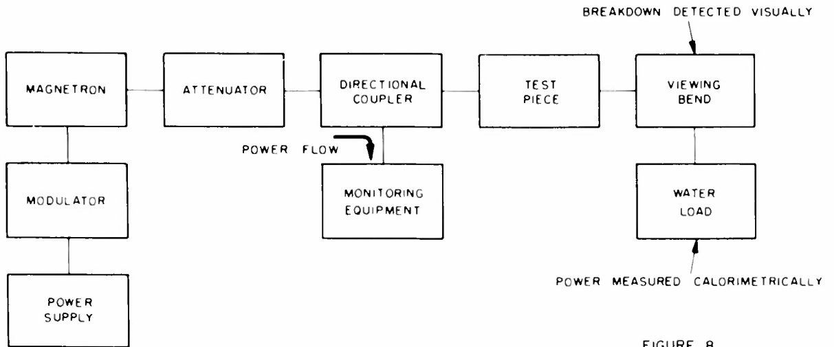
FIGURE 8 HIGH-POWER SETUP, POWER BREAKDOWN DETECTED WITH VIEWING BEND
